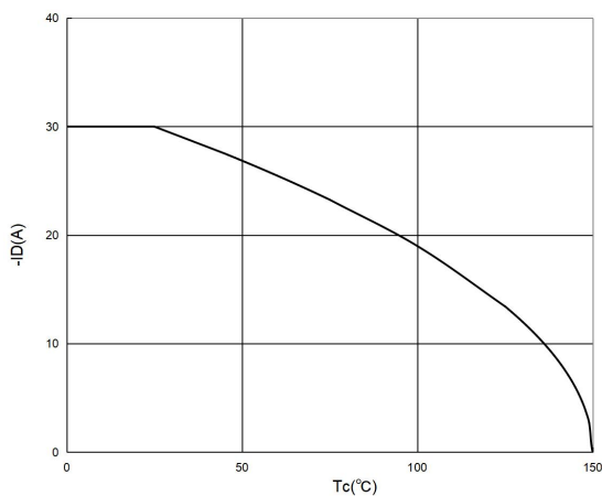
Figure 11. Current De-rating
