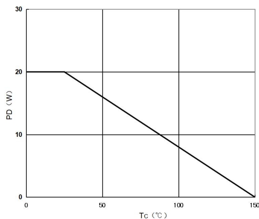
Figure 12. Power De-rating
