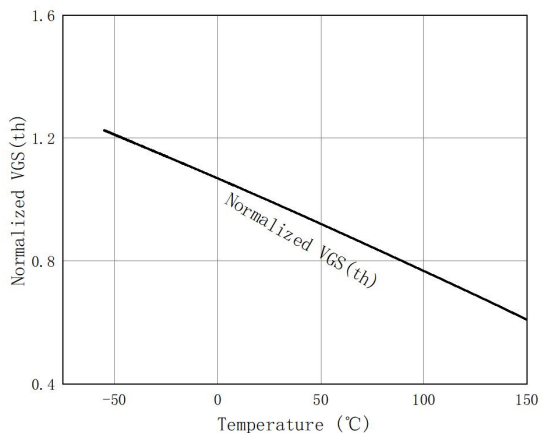
Figure 7: V_{th} vs Junction Temperature
