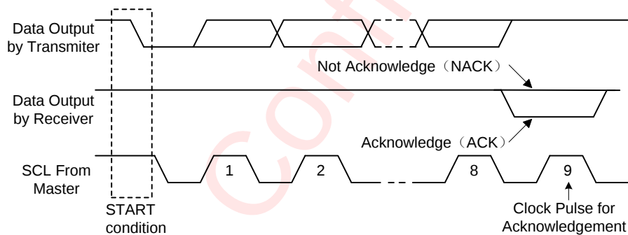
Figure 18 I²C ACK Timing
