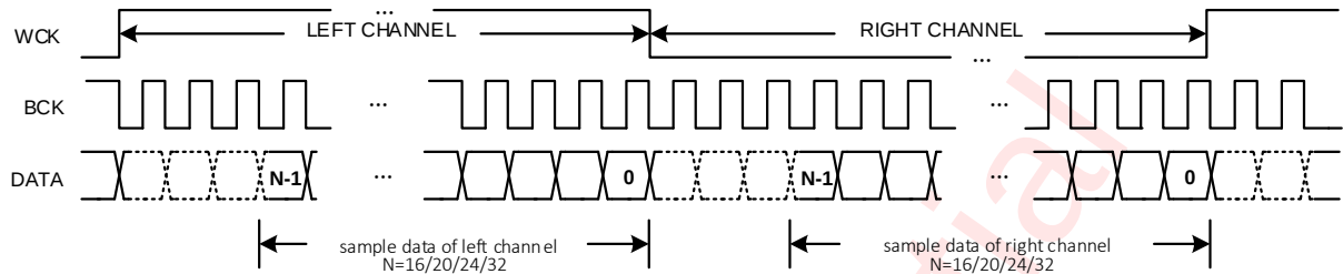
Figure 11 I²S Timing for Right-Justified Mode
