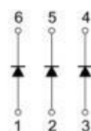
BAS70TW MARKING:K73
