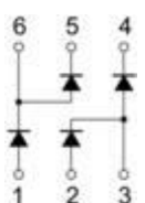
BAS70BRW MARKING:K75
