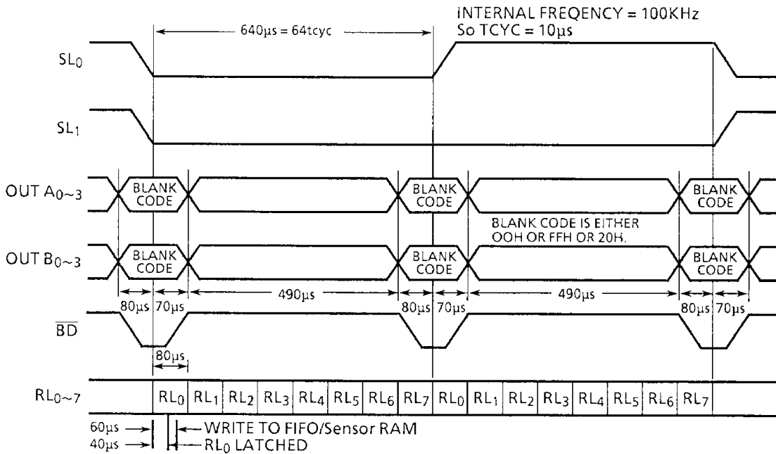
Figure 12.4 Scan Timing
