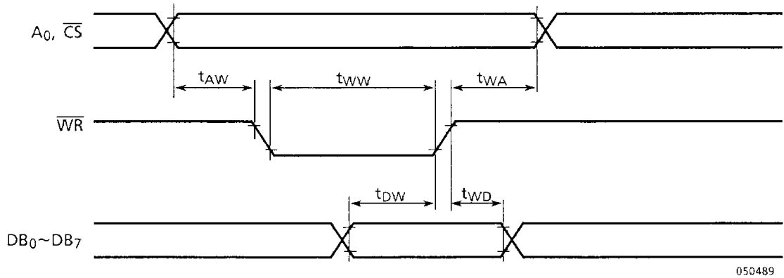
Figure 12.2 Write Timing
