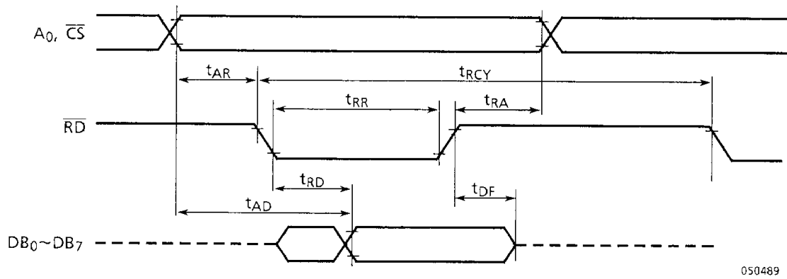
Figure 12.1 READ TIMING
