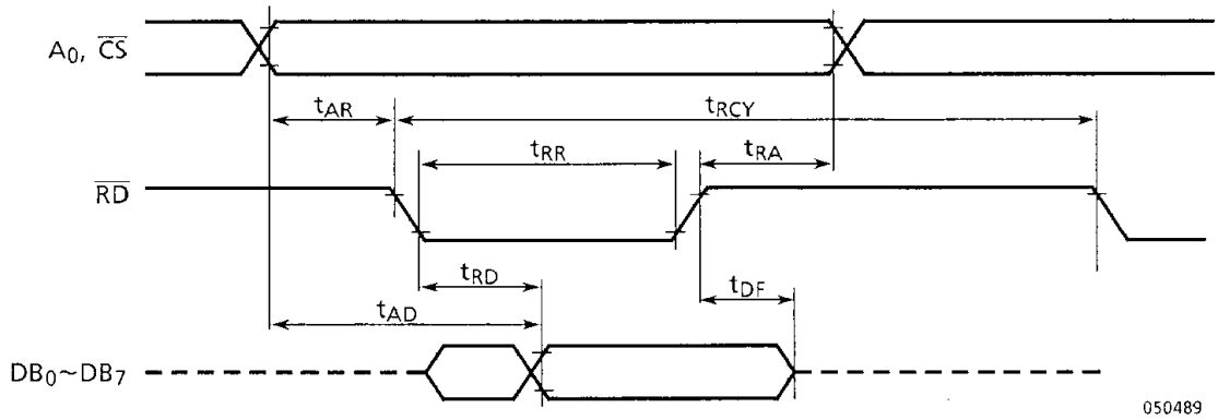
Figure 12.1 Read Timing
