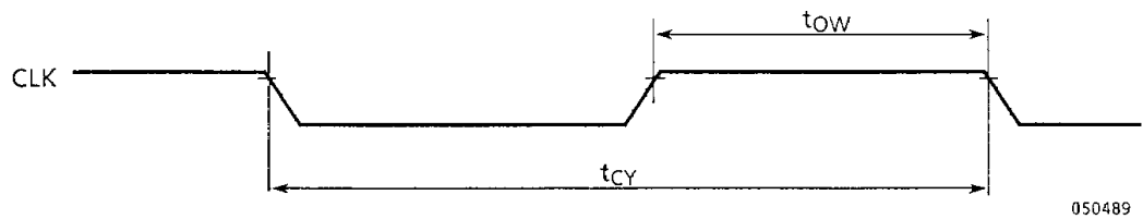
Figure 12.3 Clock Timing
