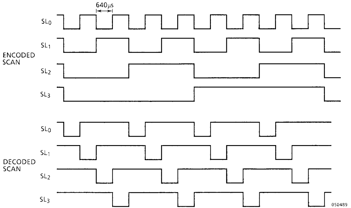
figure 12.4 scan timing
