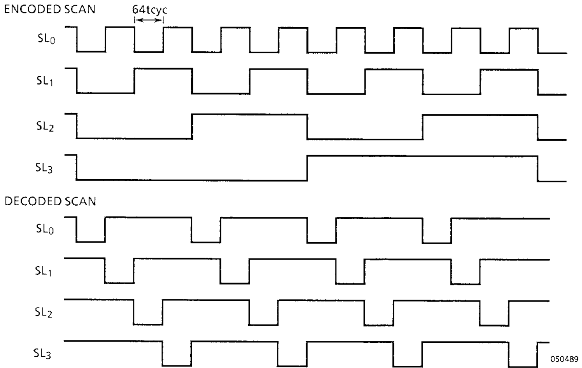
Figure 12.4 Scan Timing
