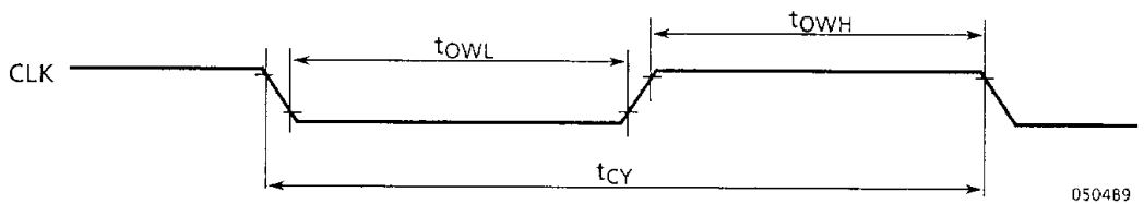
Figure 12.3 CLOCK TIMING
