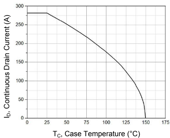
Figure 13. Drain Current vs. T_C
