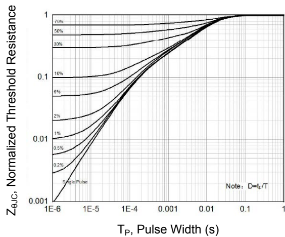
Figure 14. Transient Thermal Impedance vs. T_P
