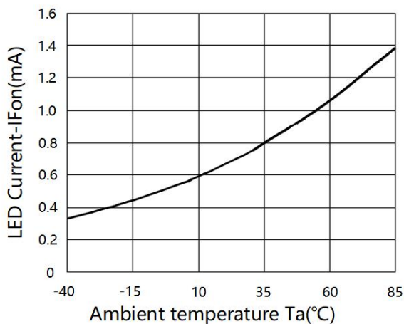
Fig.5 LED Turn On Current vs Ambient Temperature
