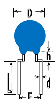
TYPE E: 平膊 Flat shoulder
