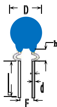
TYPE E: 平膊 Flat shoulder
