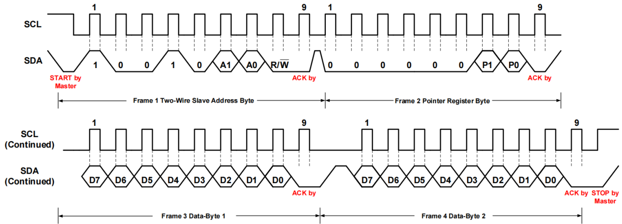
Figure 5. Two-wire Write Command Timing Diagram
