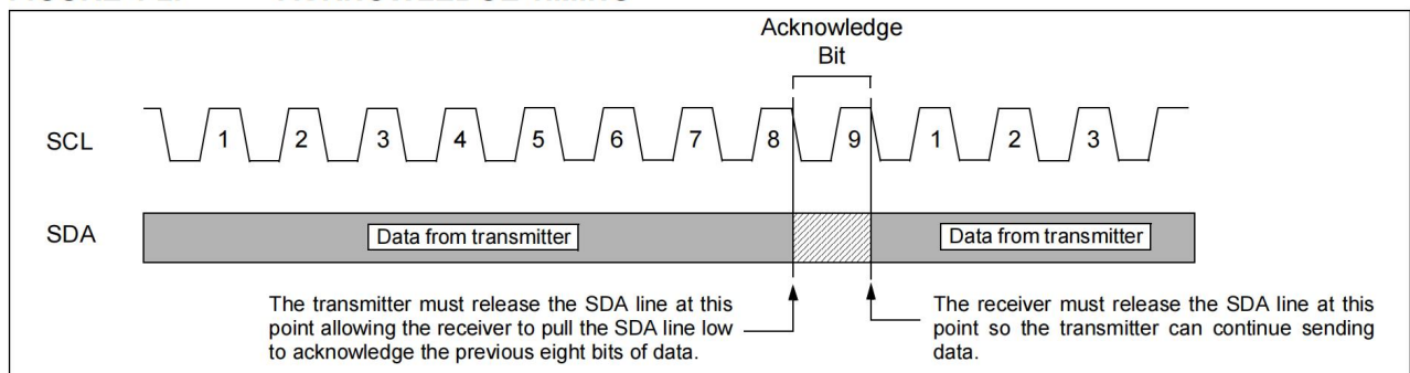
FIGURE 4-2: ACKNOWLEDGE TIMING
