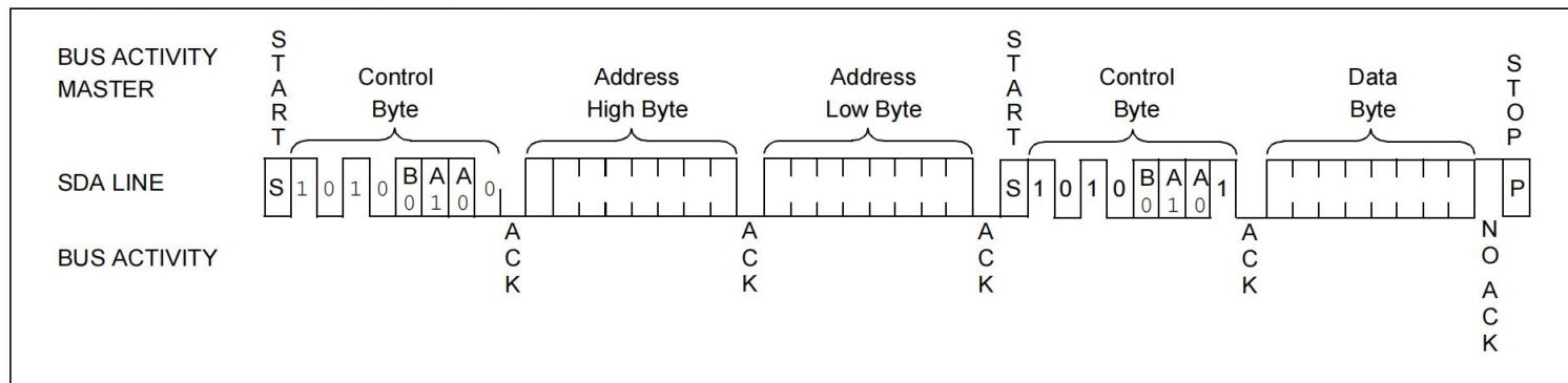
FIGURE 8-2: RANDOM READ
