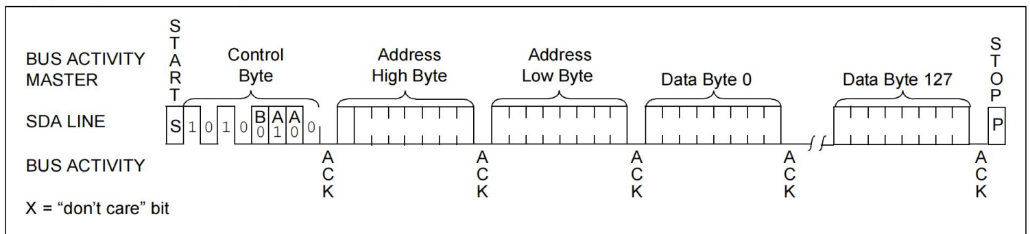
FIGURE 6-2: PAGE WRITE
