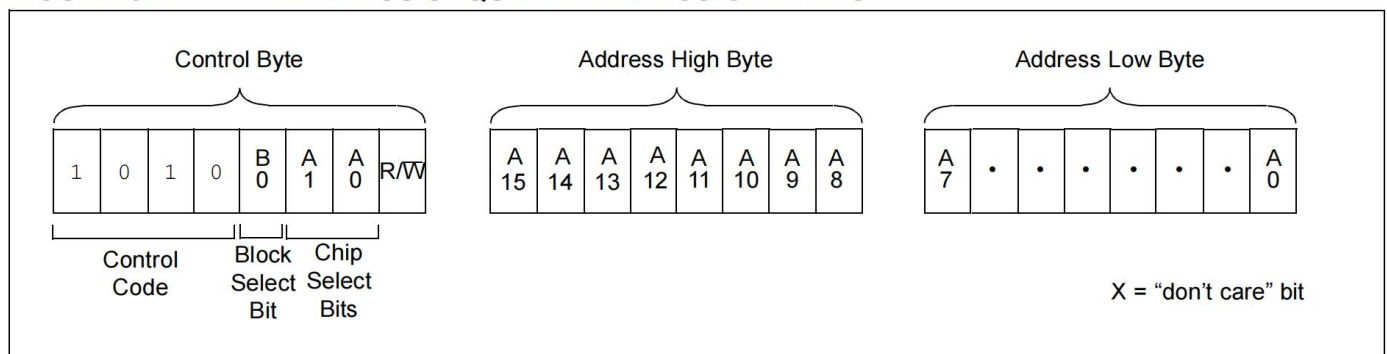
FIGURE 5-2: ADDRESS SEQUENCE BIT ASSIGNMENTS
