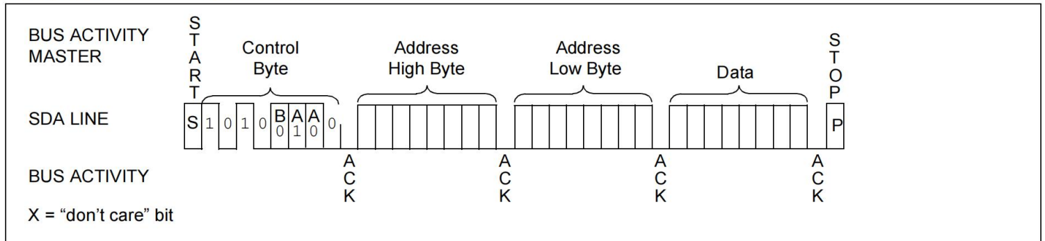
FIGURE 6-1: BYTE WRITE
