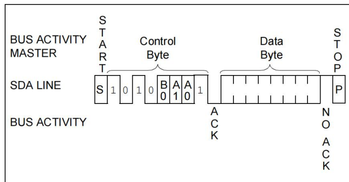
FIGURE 8-1: CURRENT ADDRESS READ
