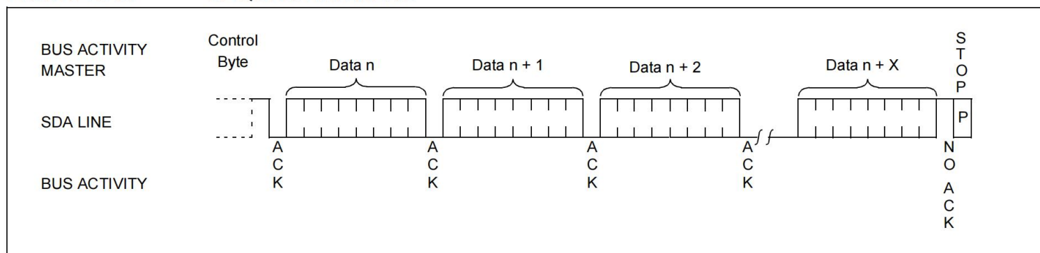
FIGURE 8-3: SEQUENTIAL READ
