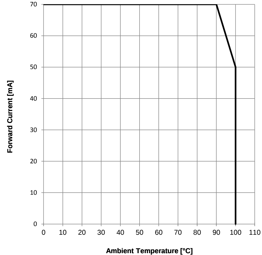
Derating Curve:
