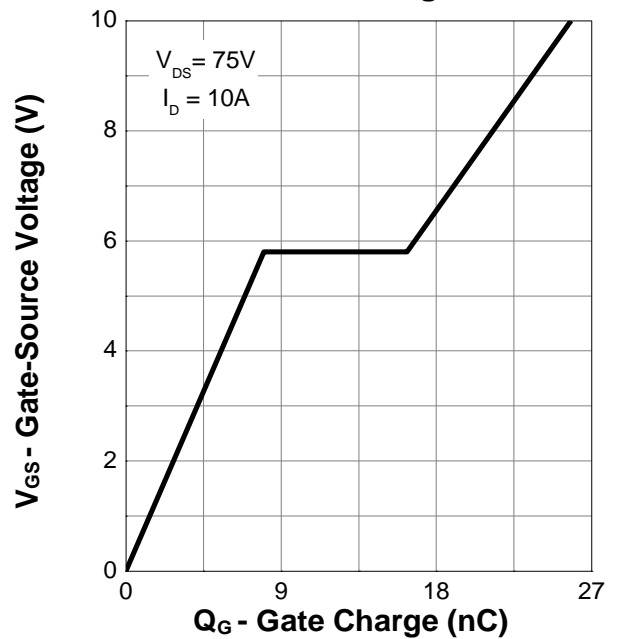
Gate Charge
