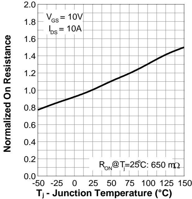
Normalized On Resistance
