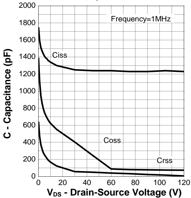
Capacitance
