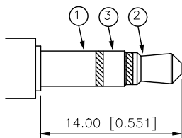
3.5 MATE PLUG
