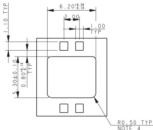
MOUNTING PCB (TOP SIDE)
