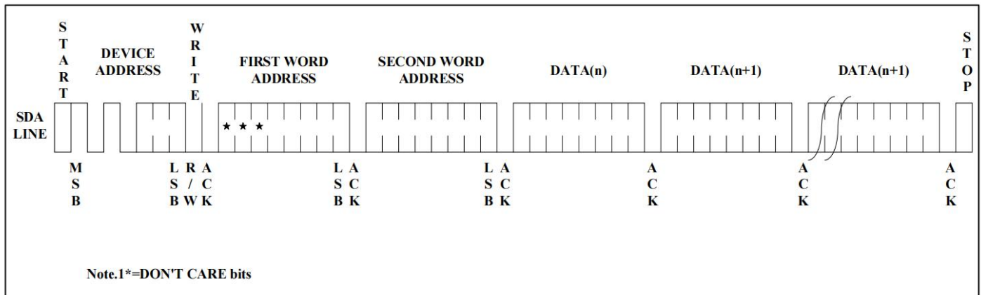
Figure 8. Page Write
