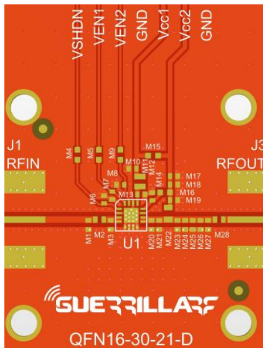
GRF5517 Evaluation Board Assembly Diagram
