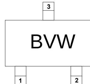
BVW= Device code Marking (Top View)
