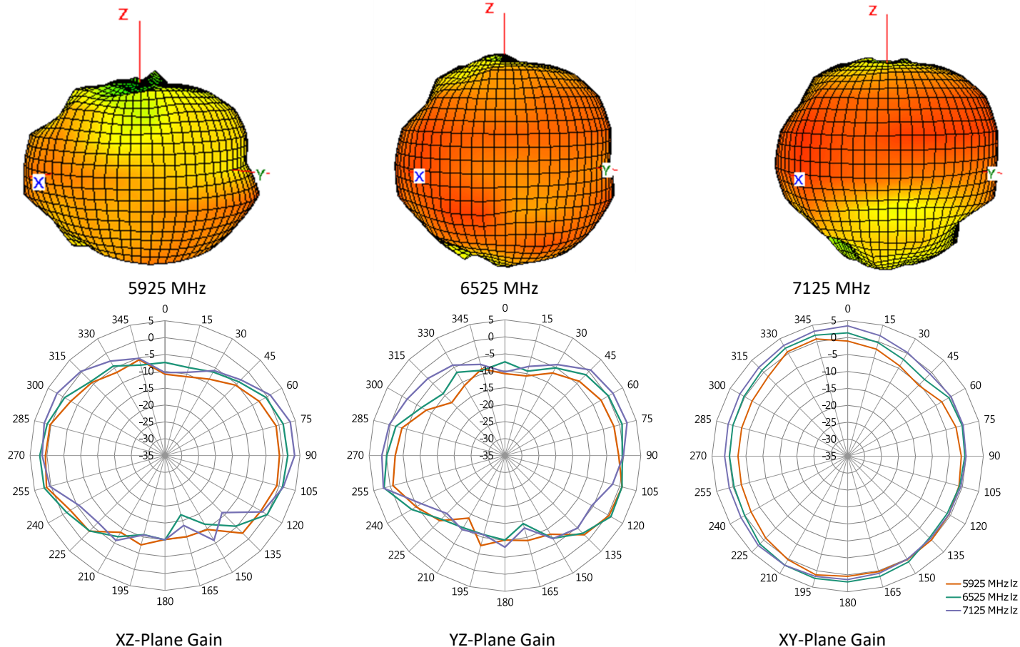
Figure 9-1. Antenna Radiation Patterns
