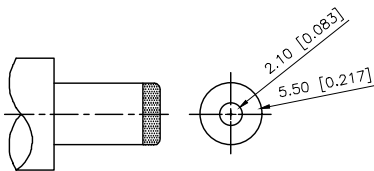
MATING PLUG Jack Insertion Depth: 9.0 mm
