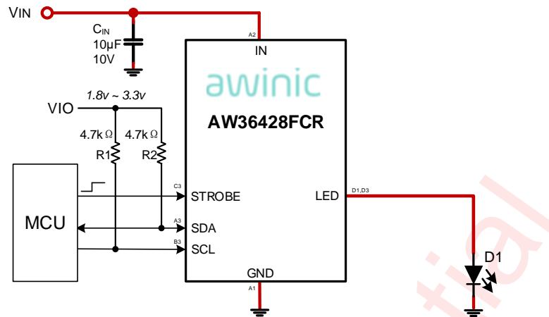
Fig 3 AW36428 Application Circuit
