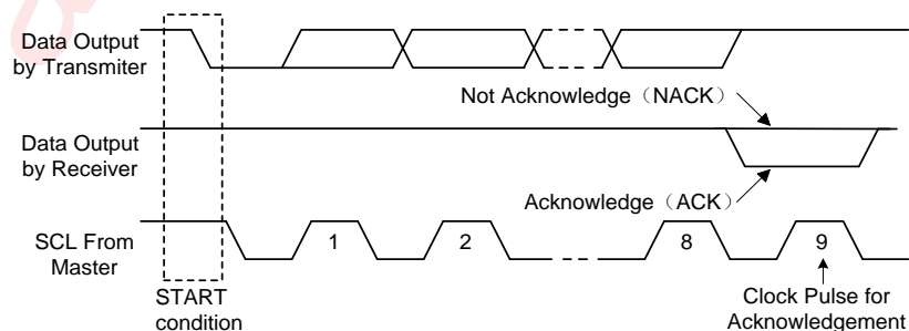
Fig 23 Acknowledgement Diagram
