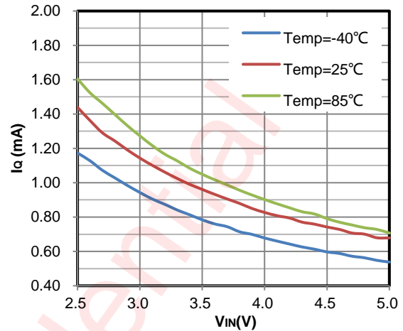
Figure 7 Iq vs. Vin, V OUT =±5.4V
