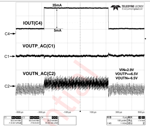
Figure 48 Load Transient (40mA Mode)
