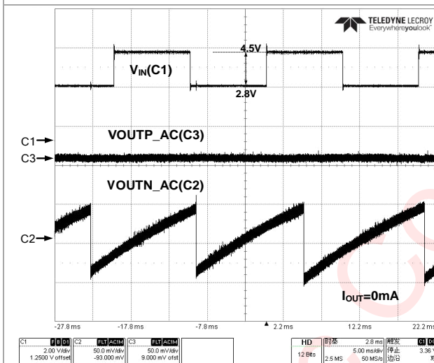
Figure 61 Line Transient (100mA Mode)
