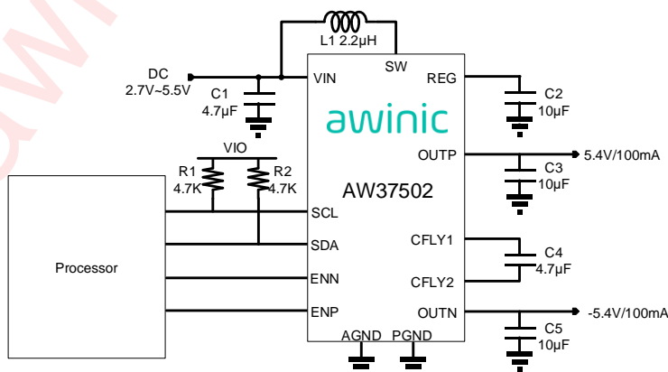
Figure 1 Typical Application Circuit of AW37502
