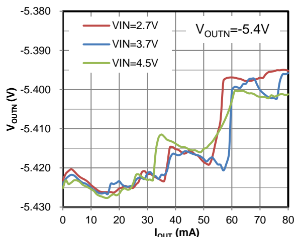
Figure 34 Load Regulation (80mA Mode)
