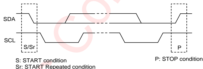
Figure 75 I 2 C Start/Stop Condition Timing
