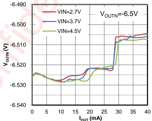
Figure 32 Load Regulation (40mA Mode)
