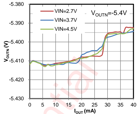
Figure 30 Load Regulation (40mA Mode)
