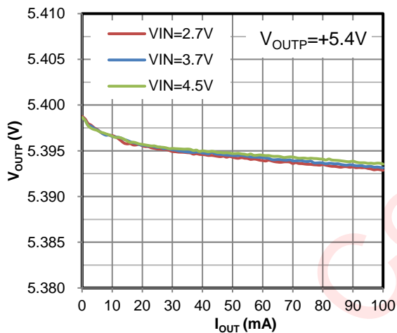
Figure 37 Load Regulation (100mA Mode)
