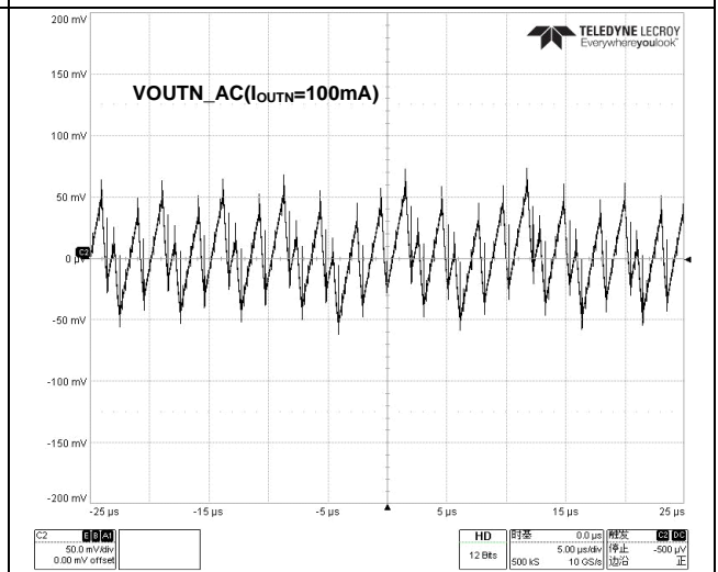
Figure 46 V OUTN Output Voltage Ripple (100mA Mode)
