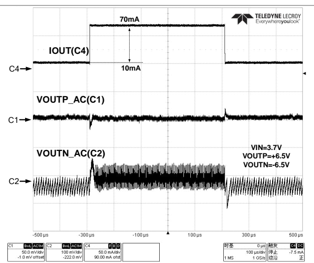
Figure 52 Load Transient (80mA Mode)
