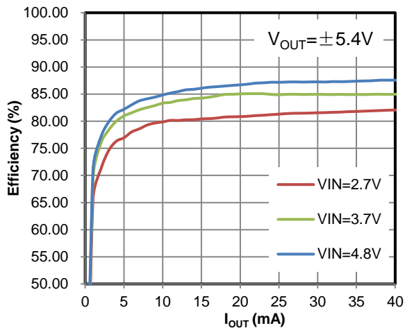
Figure 11 Efficiency (40mA Mode)
