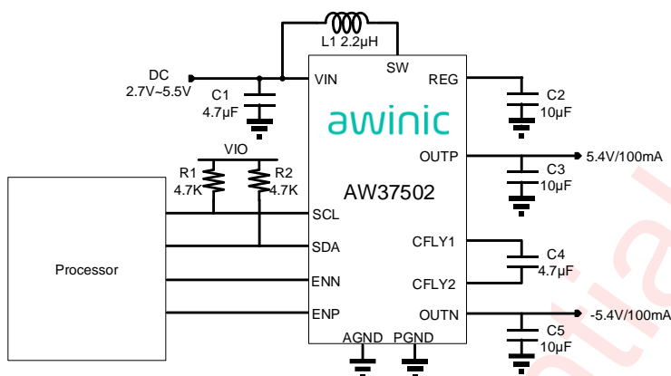
Figure 4 AW37502 Application circuit
