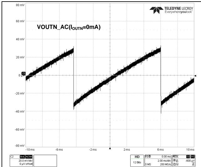
Figure 41 V OUTN Output Voltage Ripple (80mA Mode)
