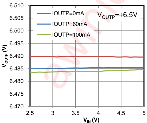
Figure 27 Line Regulation (100mA Mode)
