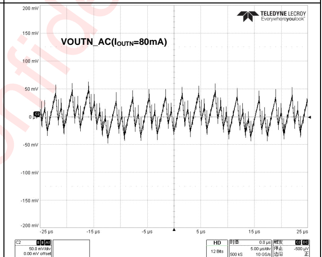
Figure 44 V OUTN Output Voltage Ripple (80mA Mode)
