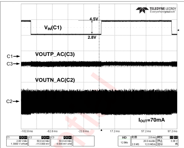
Figure 60 Line Transient (80mA Mode)
