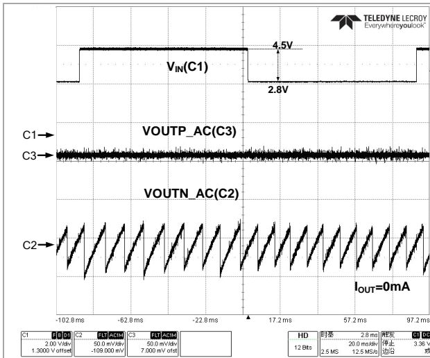
Figure 59 Line Transient (80mA Mode)
