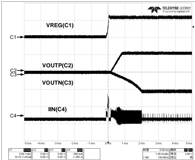
Figure 65 Inrush Current (Simultaneous)
