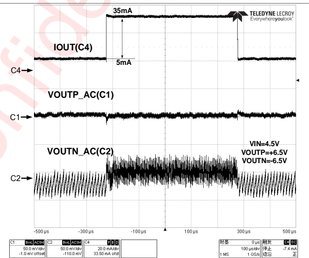
Figure 50 Load Transient (40mA Mode)
