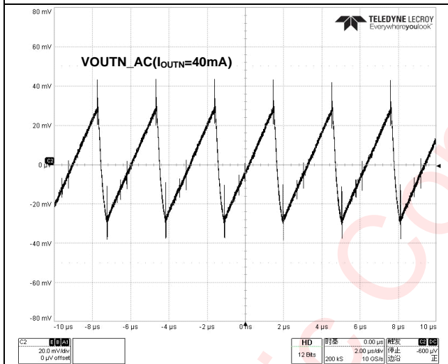
Figure 43 V OUTN Output Voltage Ripple (80mA Mode)
