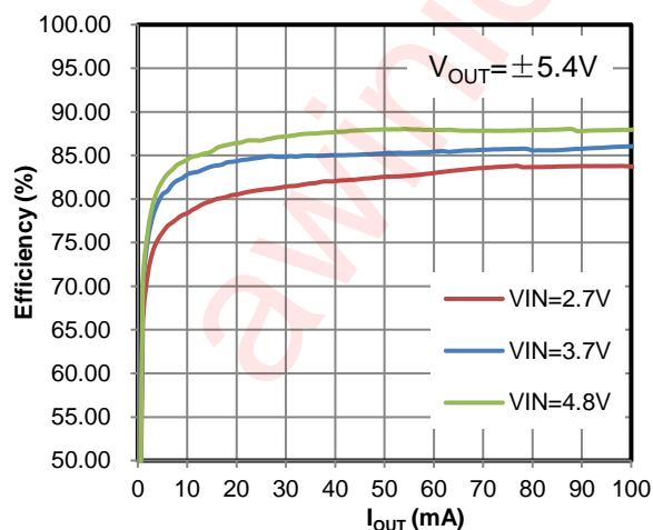
Figure 15 Efficiency (100mA Mode)
