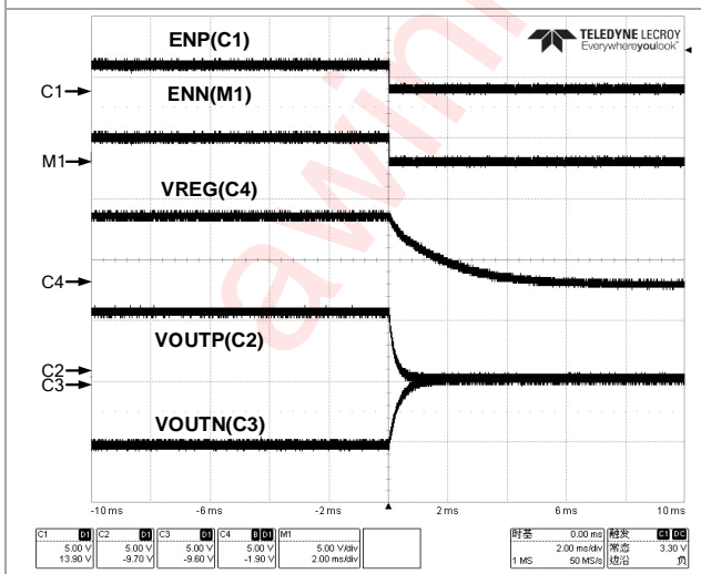
Figure 69 Power Down Sequencing (Simultaneous)
