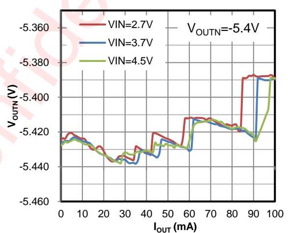
Figure 38 Load Regulation (100mA Mode)
