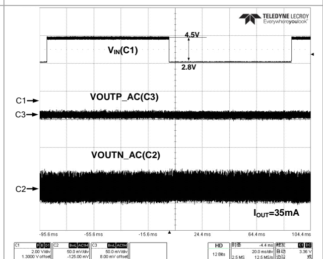
Figure 58 Line Transient (40mA Mode)
