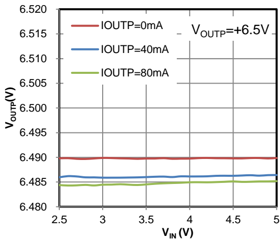
Figure 23 Line Regulation (80mA Mode)
