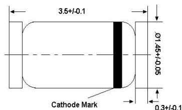
Glass case MiniMELF Dimensions in mm
