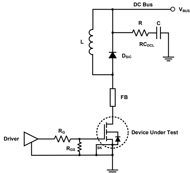
Figure 14. Switching test circuit for inductive load
