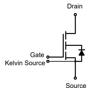
Schematic Symbol
