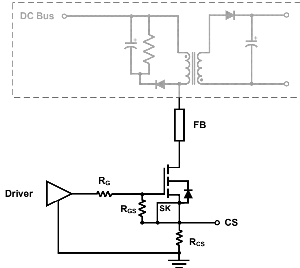
Figure 13. Simplified flyback schematic
