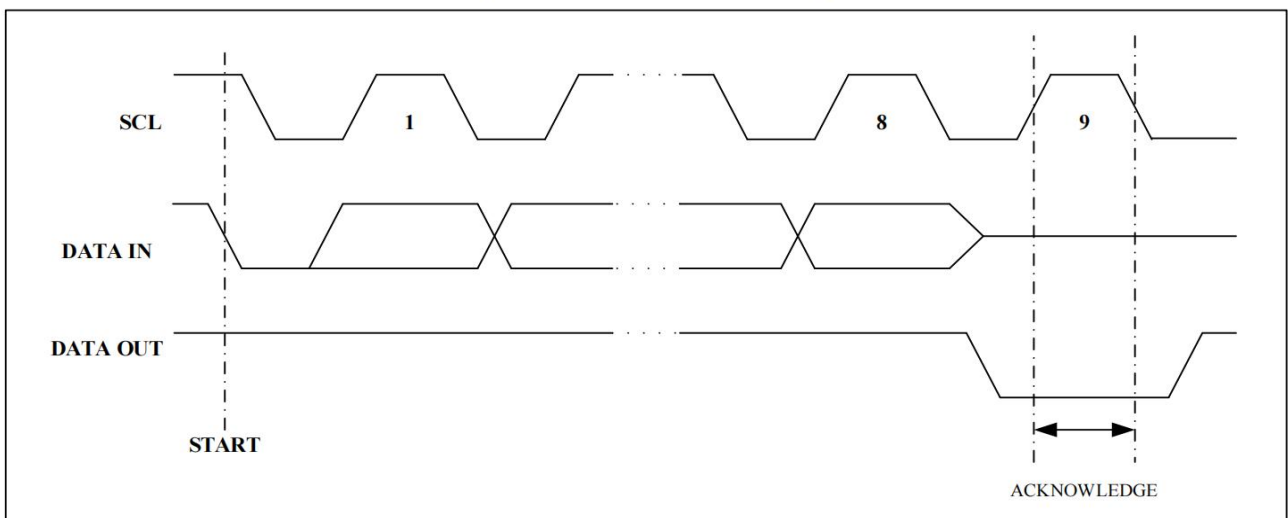
Figure 4. Output Acknowledge
