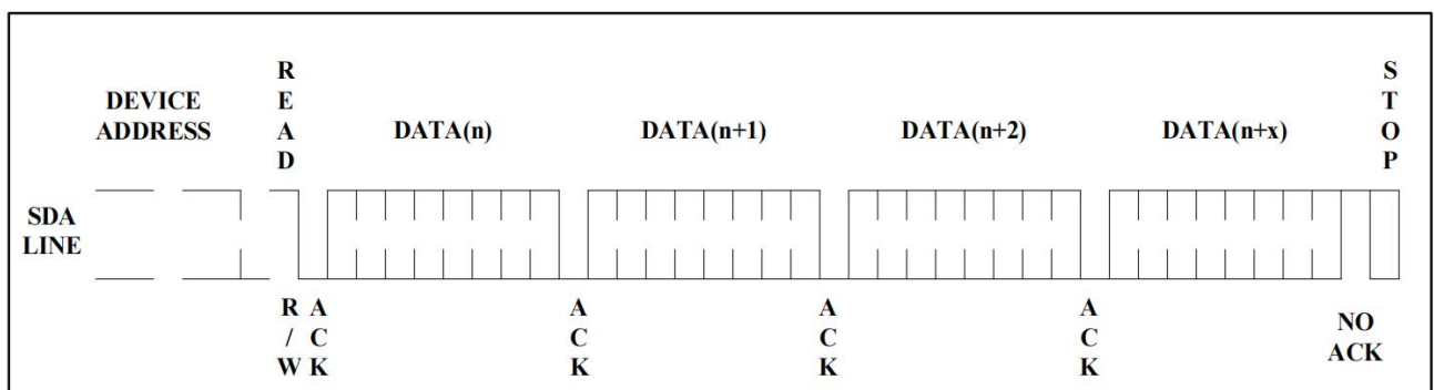
Figure 10. Sequential Read
