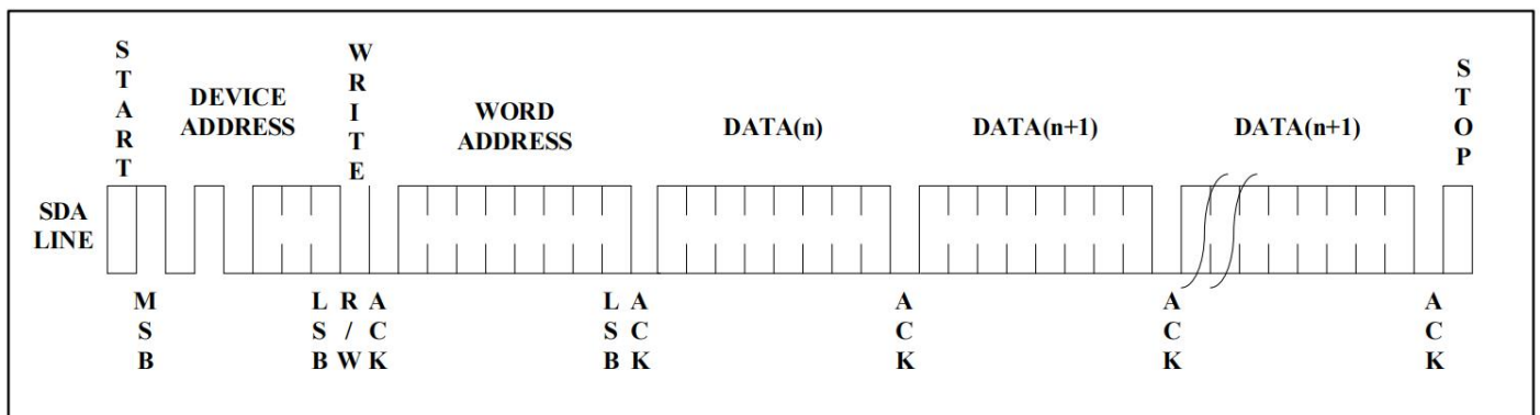
Figure 7. Page Write
