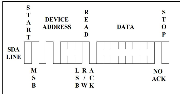
Figure 9. Random Read
