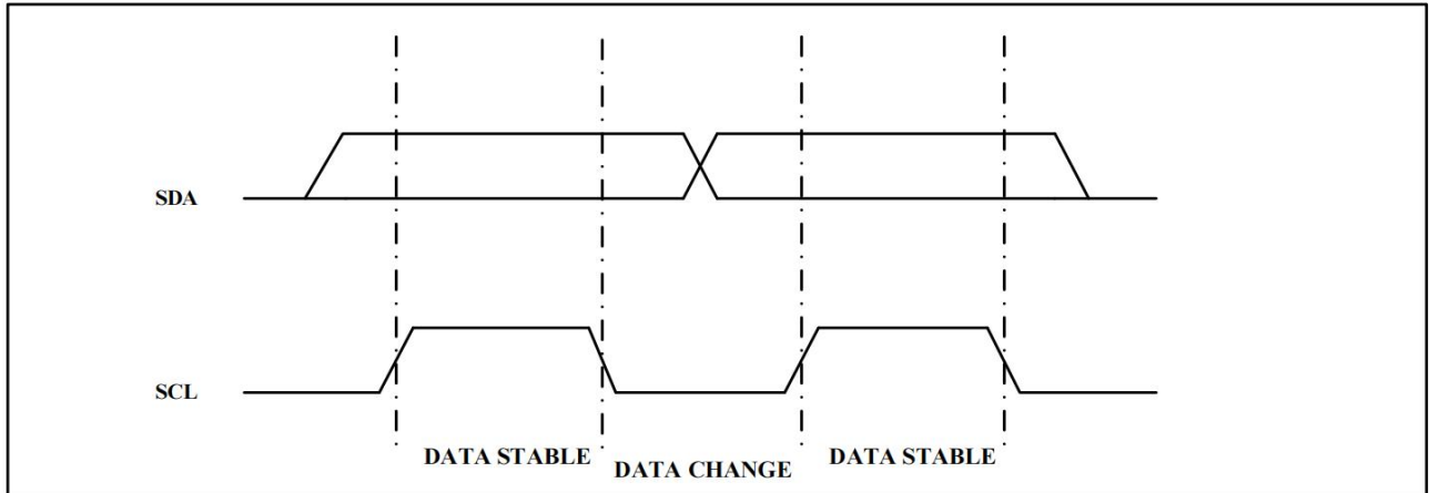
Figure 2. Data Validity
