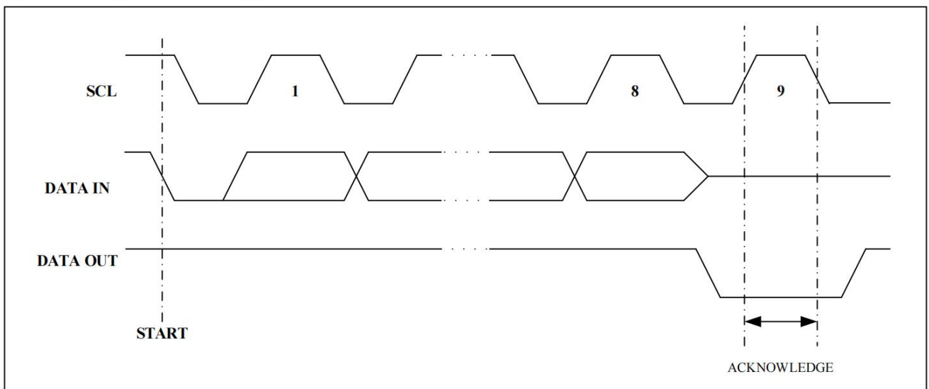
Figure 4. Output Acknowledge
