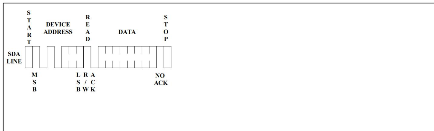
Figure 9. Random Read
