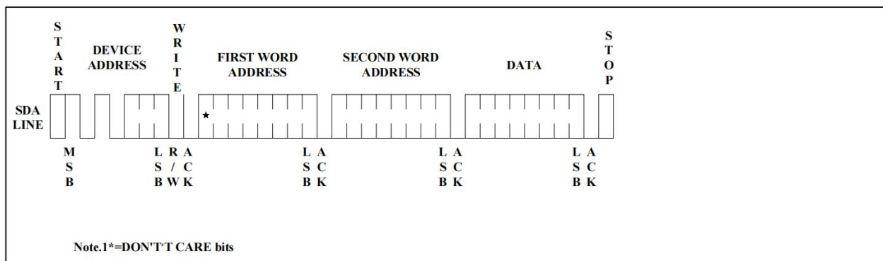
Figure 6. Byte Write
