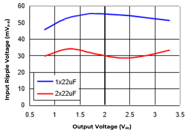
Figure 34. Input ripple voltage for various output voltages with 1x22\mu F or 2x22\mu F ceramic capacitors at the input (3A load). Input voltage is 5V.
