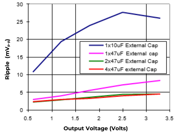
Figure 36. Output ripple voltage for various output voltages with external 1x10 µF, 1x47 µF, 2x47 µF or 4x47 µF ceramic capacitors at the output (3A load). Input voltage is 5V.
