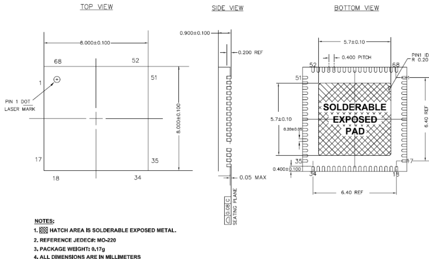
Figure 10. 68-Pin (8X8X0.90 mm) QFN (Sawn Type)
