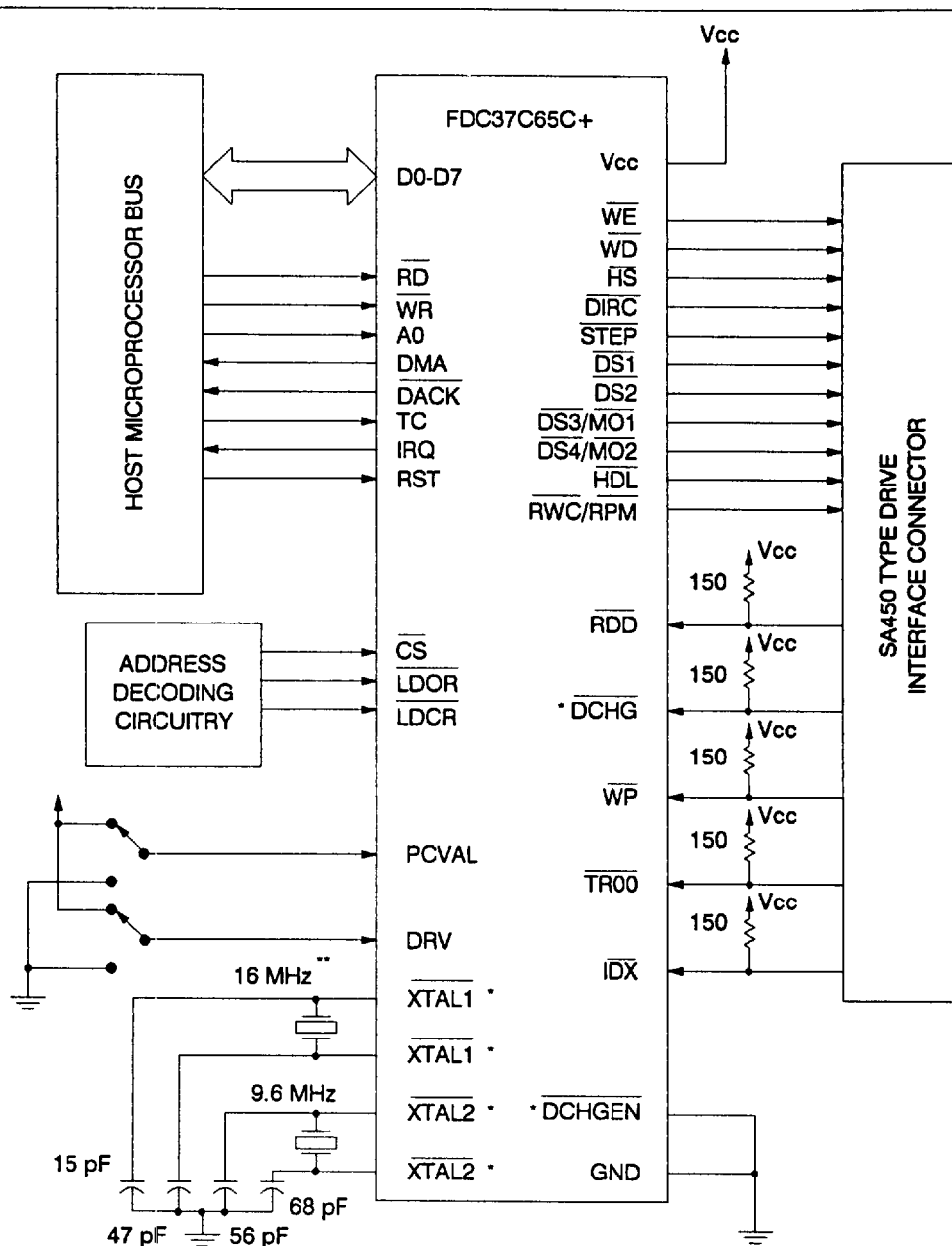
FIGURE 1 - TYPICAL SYSTEM BLOCK DIAGRAM
