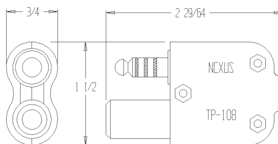
Telephone Plug Biaxial Shielded Eight Conductor
