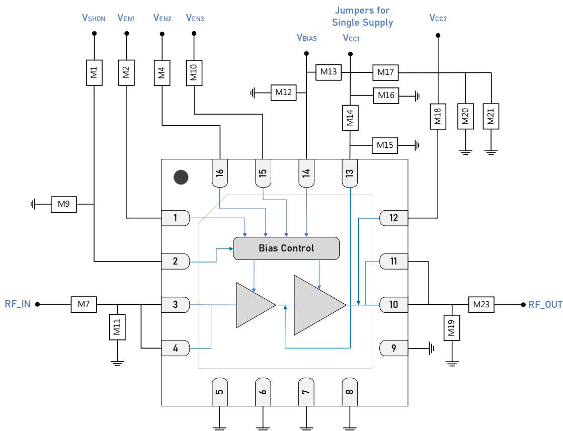
GRF5536 Standard Evaluation Board Schematic
