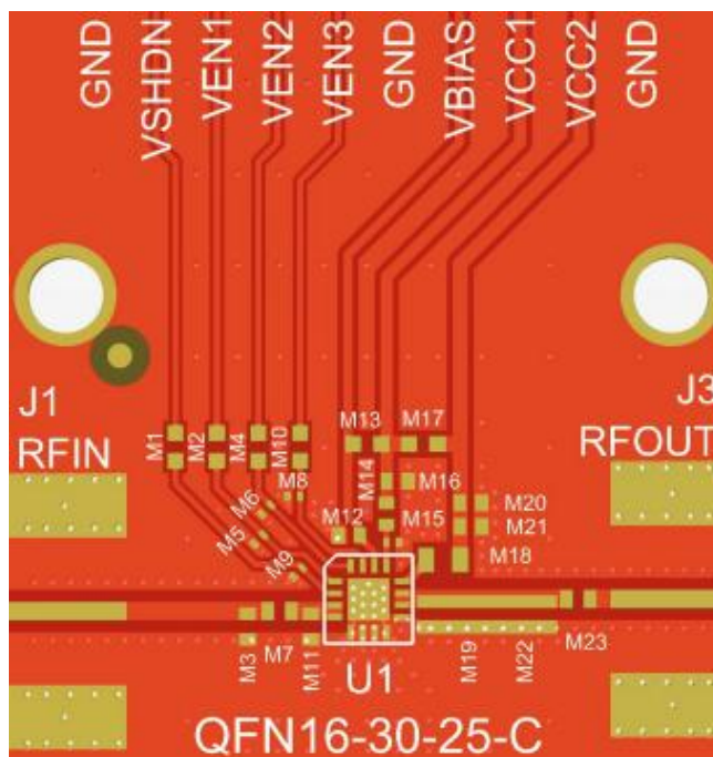
GRF5536 Evaluation Board Assembly Diagram
