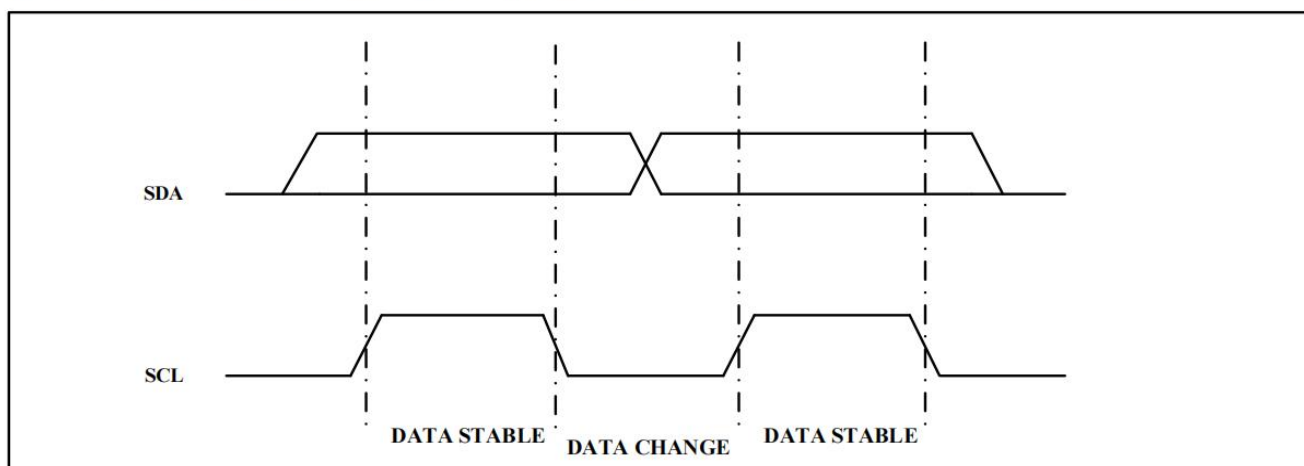
Figure 2. Data Validity
