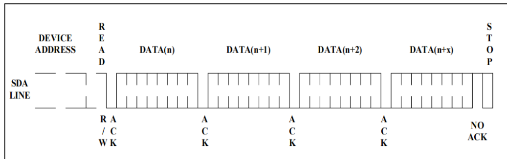
Figure 11. Sequential Read
