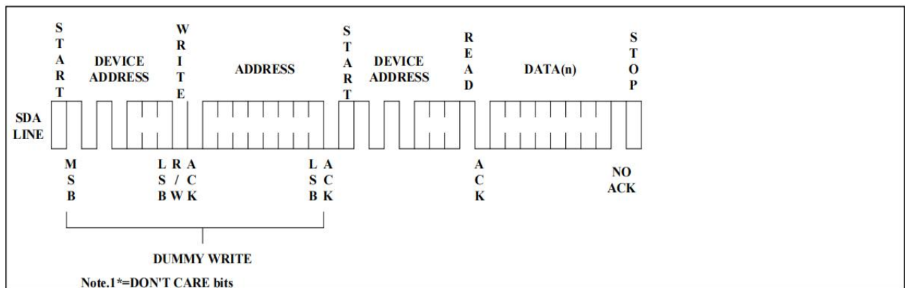
Figure 10. Random Read
