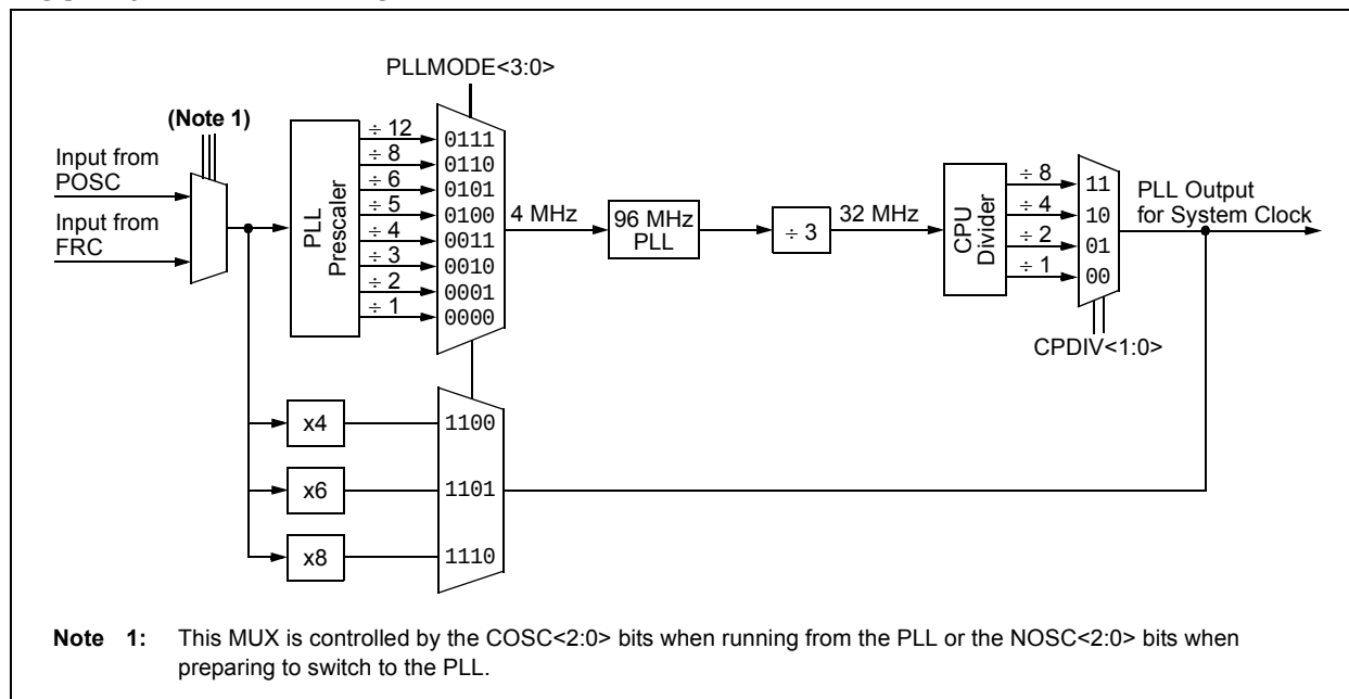
FIGURE 9-2: PLL BLOCK
