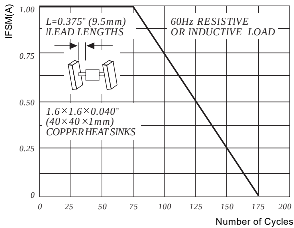
FIG5: Maximum Non-Repertive Surge Current
