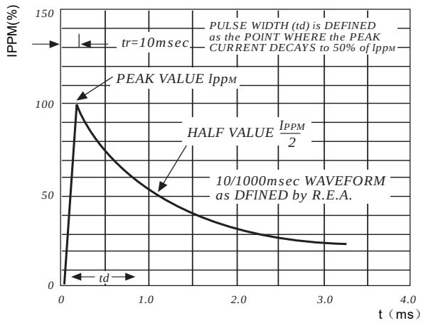
FIG5: Maximum Non-Repertive Surge Current
