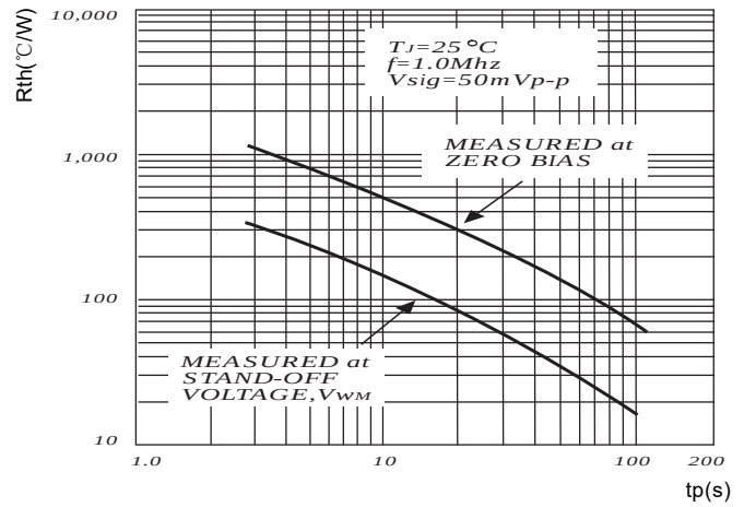
FIG4: Typical Transient Thermal Impedance
