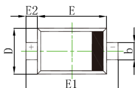
SOD523Package Outline
