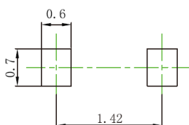
Land Pattern Recommendation
