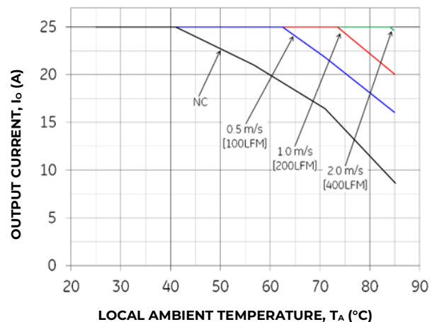
Figure 21. Output Current Derating for the Base plate QBVW033A0B-H at 48V in with 0.25" heatsink and ransverse airflow from V_{in}(-) to V_{in}(+)
