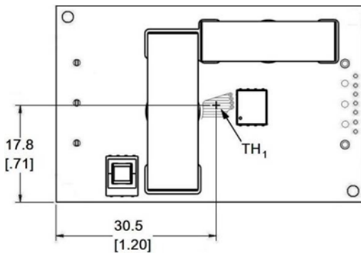
Figure 17. Location of the thermal reference temperature TH1 for open-frame modules.
