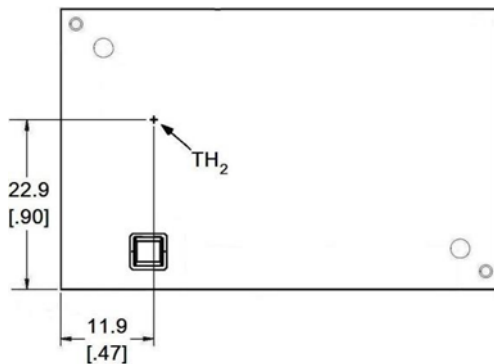
Figure 18. Location of the thermal reference temperature TH2 for baseplate modules
