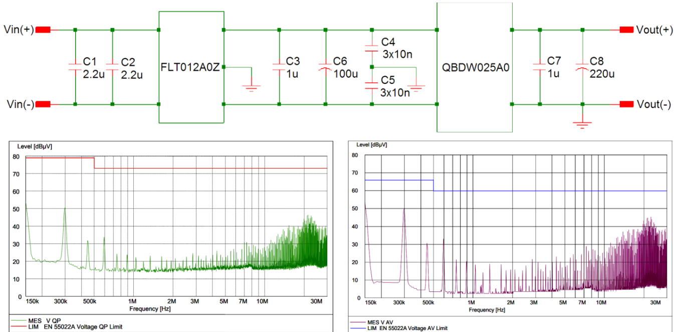
Figure 25. EMC Consideration
