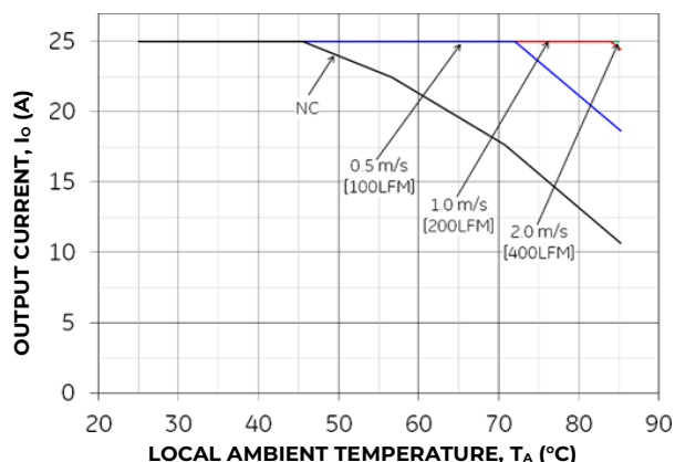
Figure 22. Output Current Derating for the Base plate QBVW033A0B-H at 48V in with 0.5" heatsink and Transverse airflow from V_{in}(-) to V_{in}(+)
