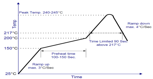
Figure 24. Recommended linear reflow profile using Sn/Ag/Cu solder.
