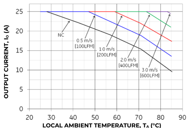
Figure 19. Output Current Derating for the Open Frame QBVW033A0B at 48V in with Transverse airflow from V_{in}(-) to V_{in}(+)
