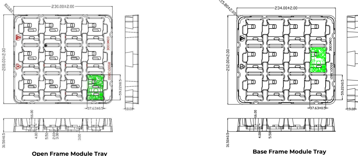
Figure 26. QBDW033 Packaging Tray
