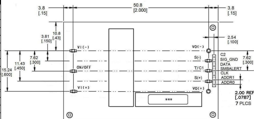
BOTTOM VIEW
