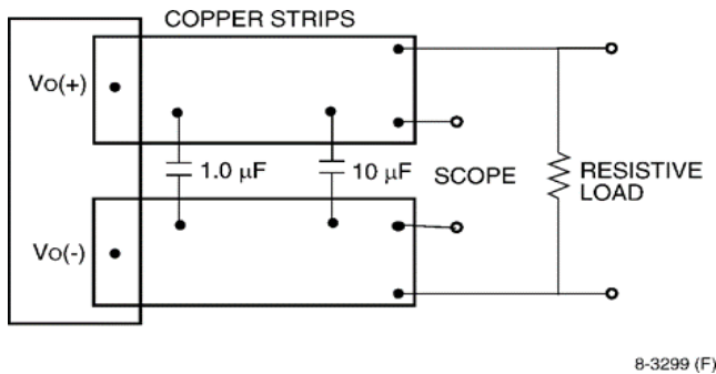
Figure 12. Output Ripple and Noise Test Setup.
