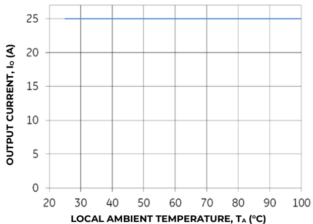
Figure 24. Output Current Derating for the Base Plate QBVW033A0B-H at 48V in in a Cold wall application; Local Internal Air Temperature near module=80°C; VOUT setting anywhere from 6.0V to 12.0V
