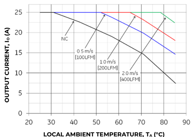
Figure 20. Output Current Derating for the Base plate QBVW033A0B-H at 48V in with Transverse airflow from V_{in}(-) to V_{in}(+)
