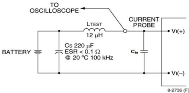
Figure 11. Input Reflected Ripple Current Test Setup
