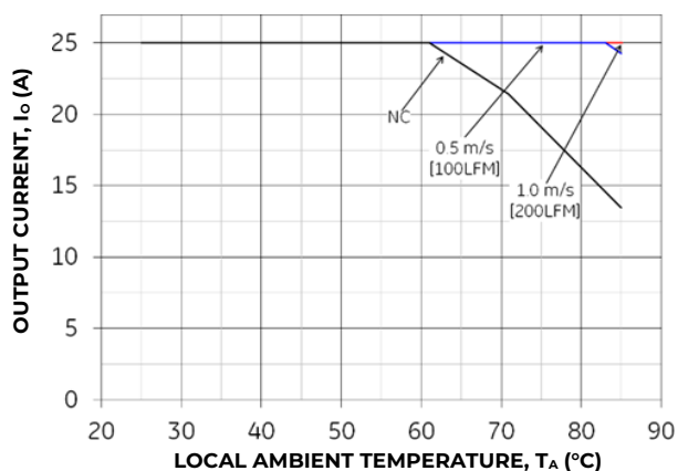
Figure 23. Output Current Derating for the Base plate QBVW033A0B-H at 48V in with 1.0" heatsink and Transverse airflow from V_{in}(-) to V_{in}(+)
