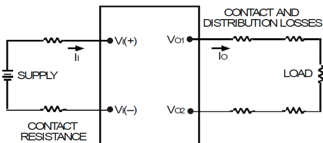
Figure 13. Output Voltage and Efficiency Test Setup.
