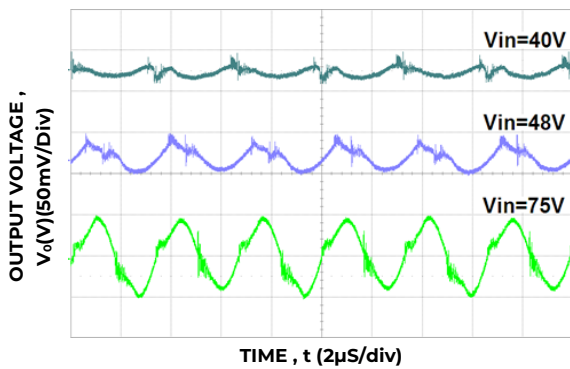
Figure 3. Typical Output Ripple and Noise, I_o = I_{o,max} .
