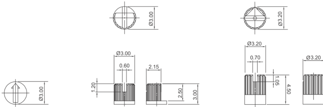
B: KNURLED, SLOTTED, FLATTED SHAFT
