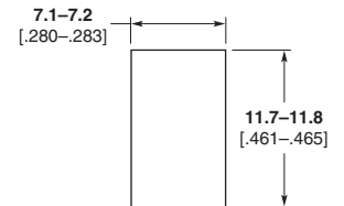
Recommended Panel Cutout Panel Thk. 1.2/1.7 [0.047/0.067]
