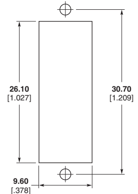
Recommended Panel Cutout Max. Panel Thk. 1.7 [0.067]
