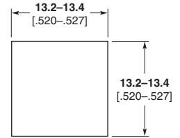
Recommended Panel Cutout Panel Thk. 1.2/1.7 [0.047/0.067]
