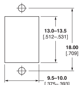
Recommended Panel Cutout Max. Panel Thk. 1.70 [.067]
