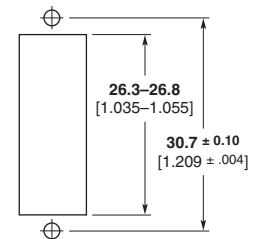
Recommended Panel Cutout Max. Panel Thk. 1.7 [0.067]
