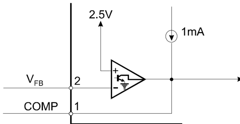
Figure 1. Error Amp Configuration
