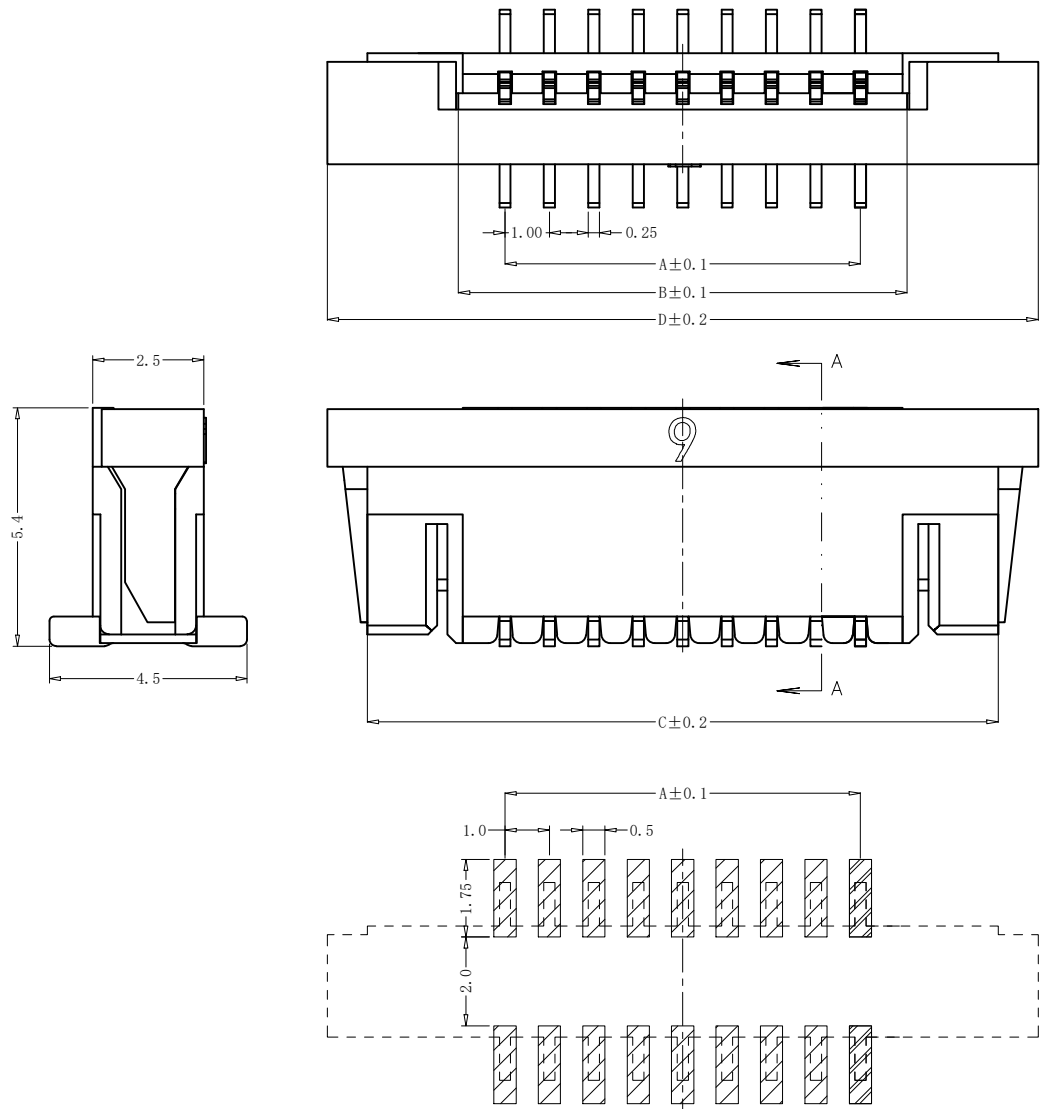
PCB LAYOUT
