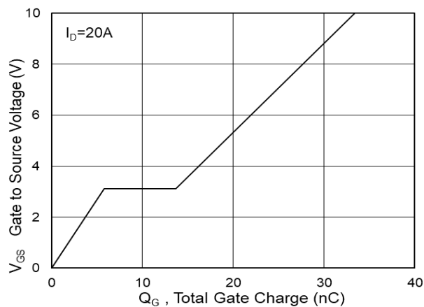
Fig.4 Gate-Charge Characteristics
