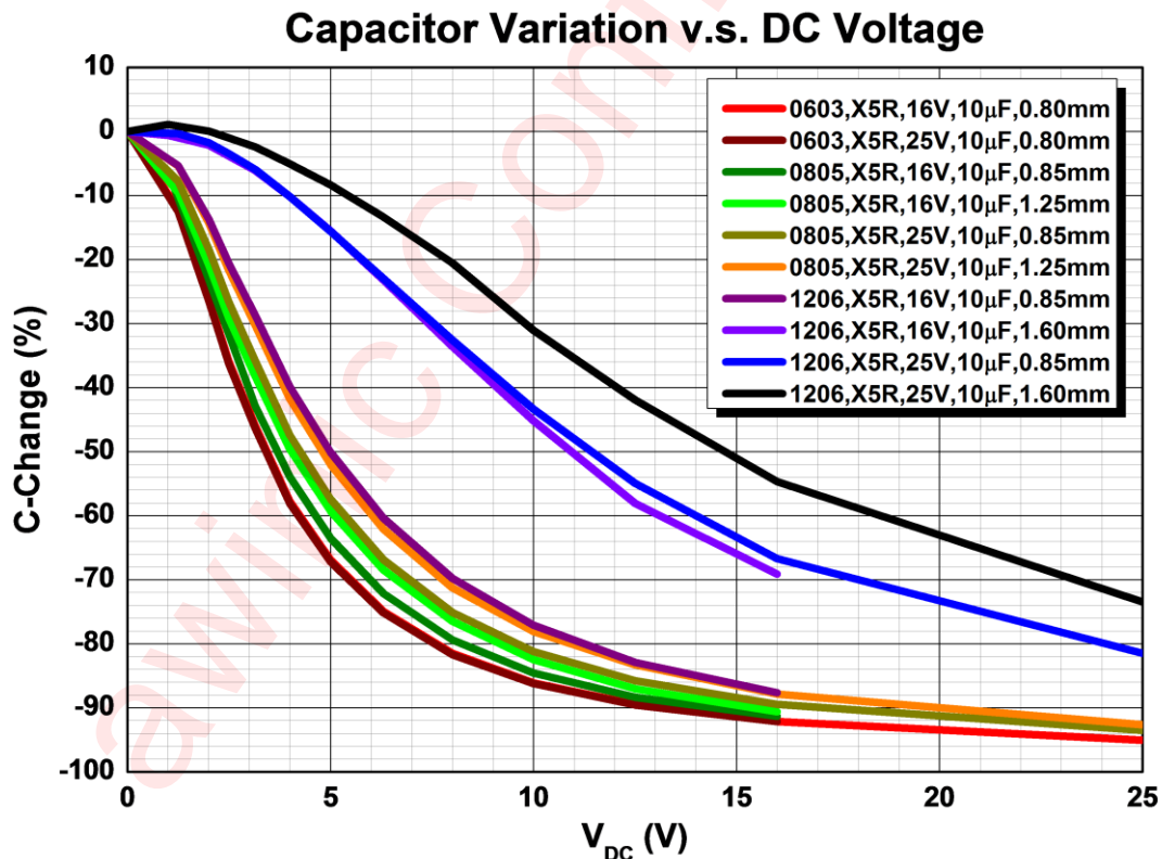
Figure 24 Different Types of Capacitive Voltage Stability
