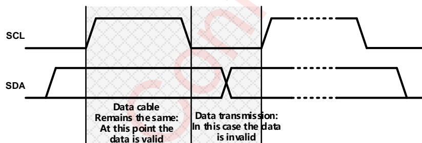
Figure 20 The Data Transfer Rules on the I²C Bus
