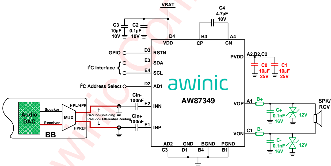
Figure 5 AW87349 Speaker & Receiver 2-in-1 Mode Application Diagram
