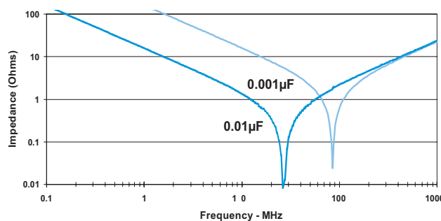
Figure 10. Impedance vs Frequency for C0G Dielectric
