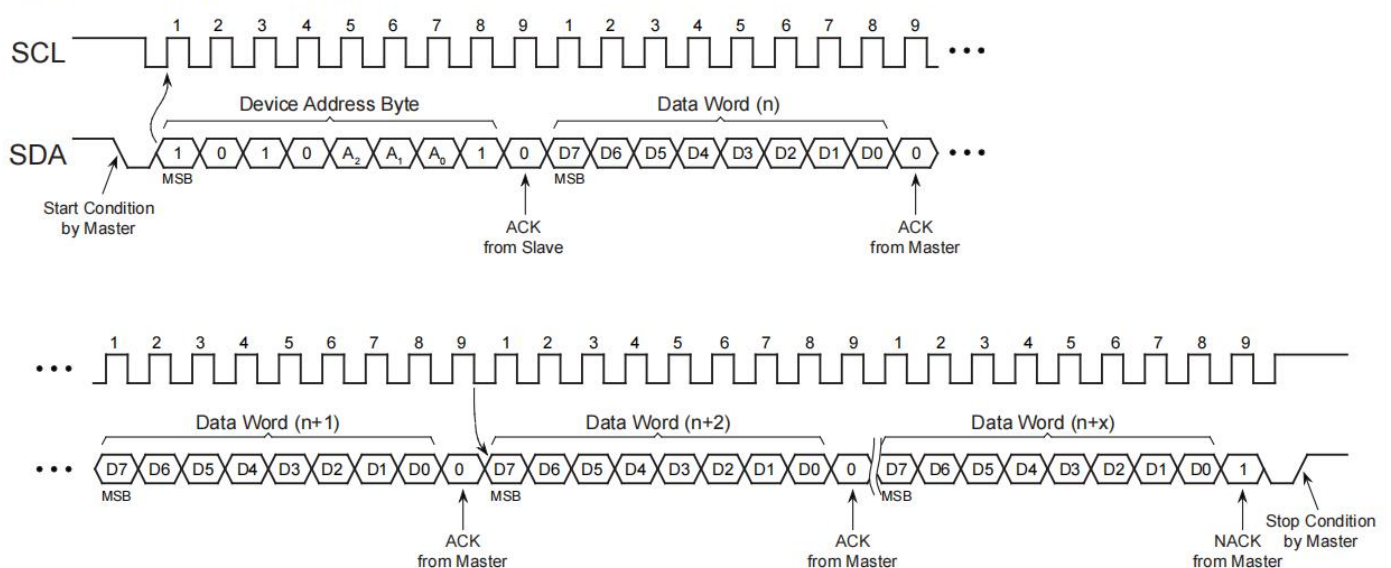
Figure 8-3. Sequential Read
