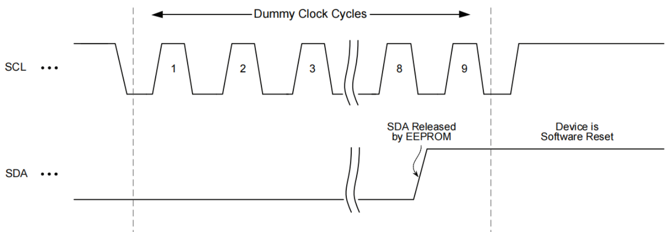
Figure 5-2. Software Reset
