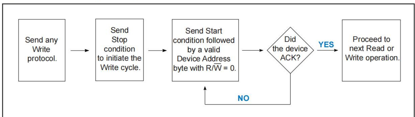
Figure 7-3. Acknowledge Polling Flowchart
