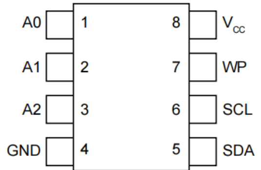
8-Lead SOIC/TSSOP
