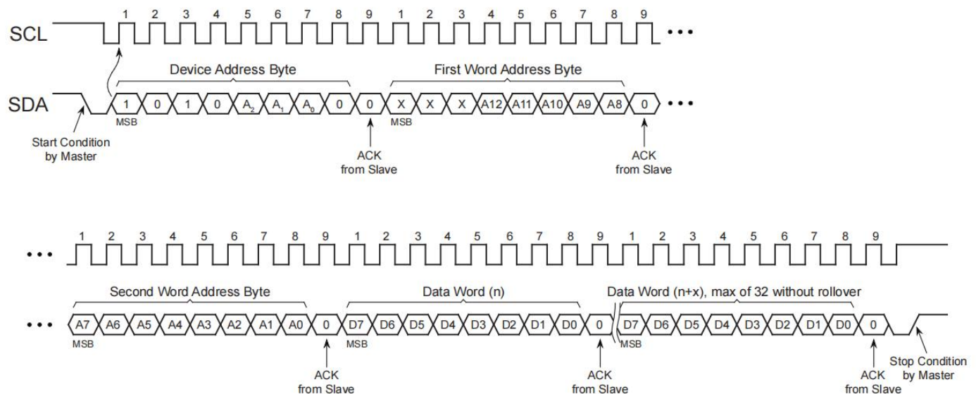
Figure 7-2. Page Write
