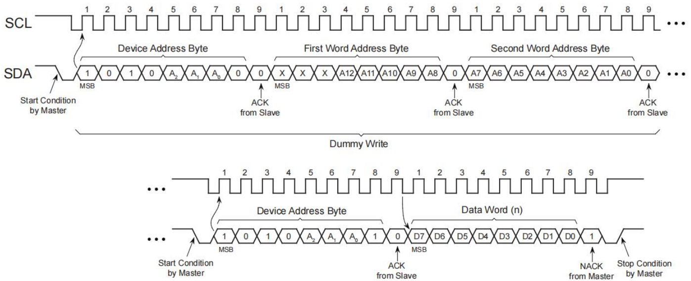
Figure 8-2. Random Read
