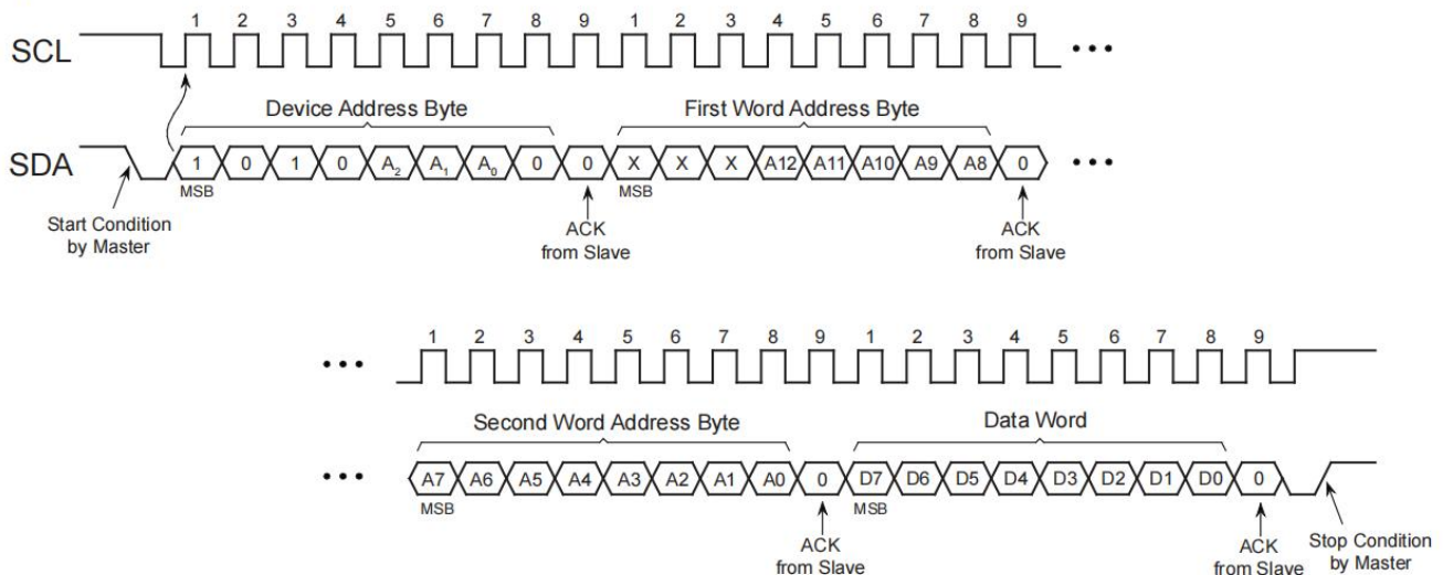
Figure 7-1. Byte Write
