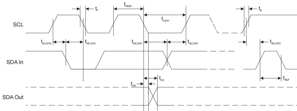
Figure 4-1. Bus Timing
