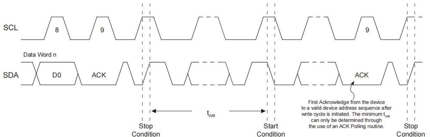
Figure 7-4. Write Cycle Timing
