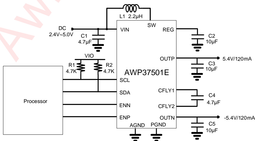
Figure 1 Typical Application Circuit of AWP37501E
