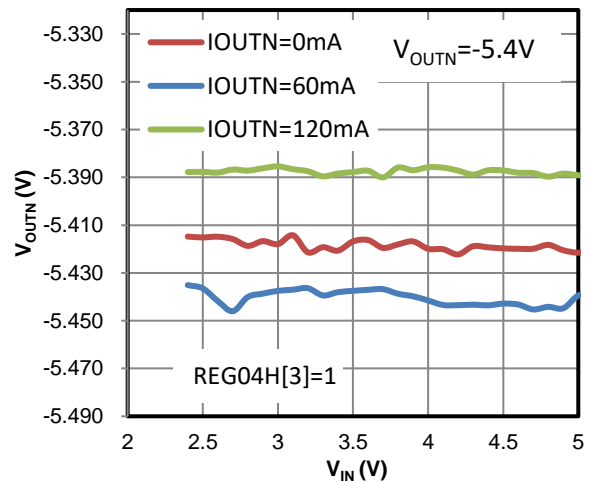
Figure 23 Line Regulation (120mA Mode)
