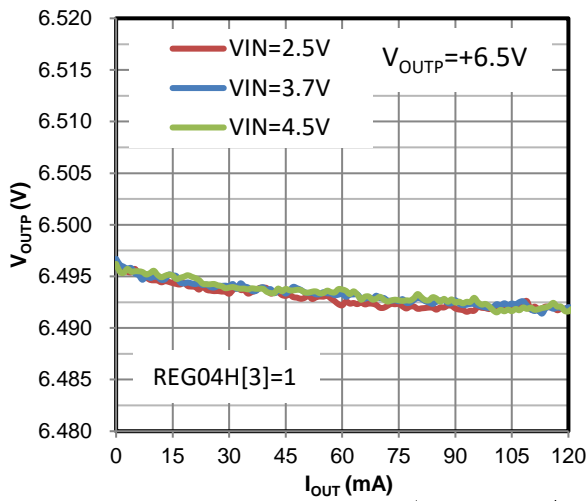
Figure 36 Load Regulation (120mA Mode)
