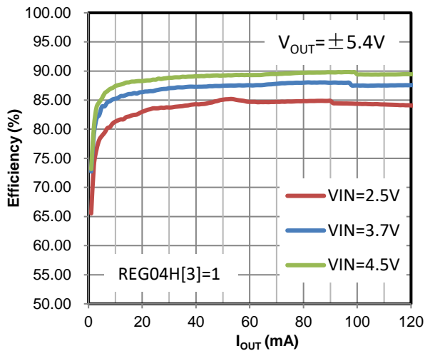
Figure 12 Efficiency (120mA Mode)
