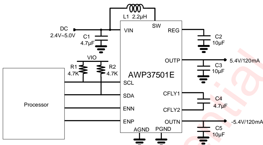
Figure 4 AWP37501E Application Circuit
