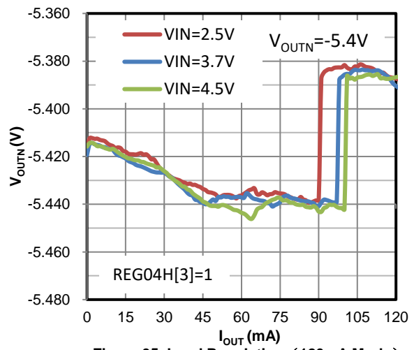
Figure 35 Load Regulation (120mA Mode)
