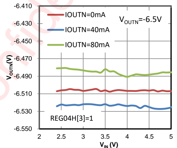
Figure 21 Line Regulation (80mA Mode)
