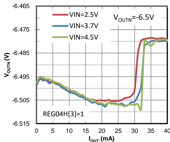
Figure 29 Load Regulation (40mA Mode)
