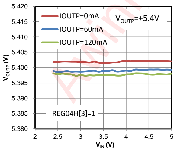
Figure 22 Line Regulation (120mA Mode)
