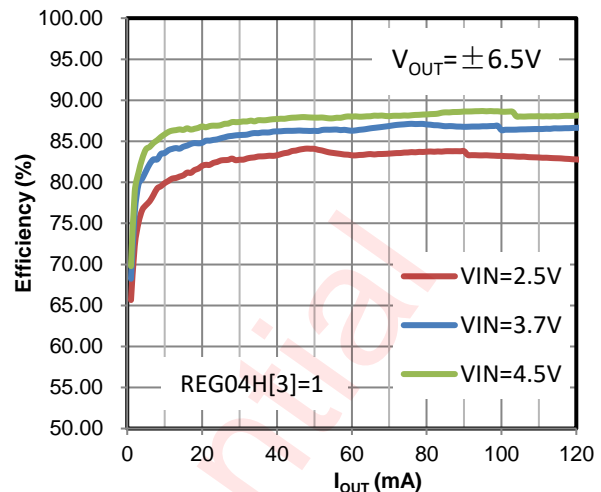
Figure 13 Efficiency (120mA Mode)
