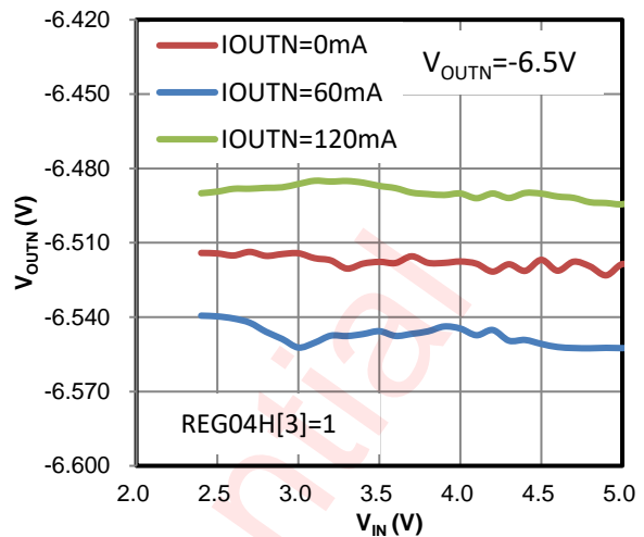
Figure 25 Line Regulation (150mA Mode)
