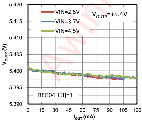
Figure 34 Load Regulation (120mA Mode)
