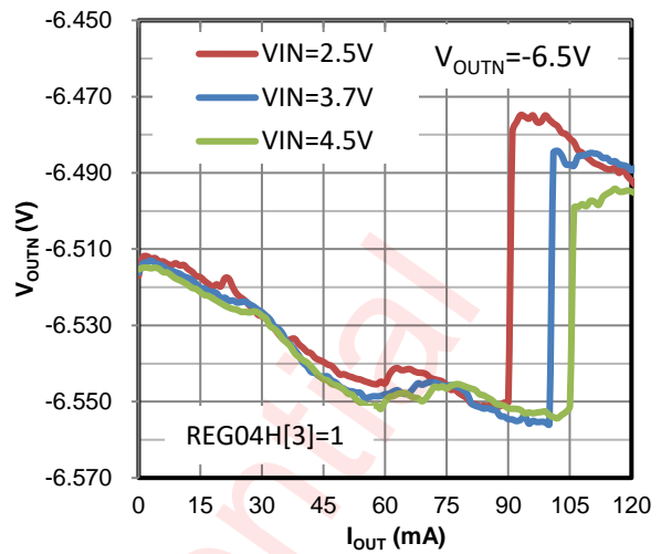
Figure 37 Load Regulation (120mA Mode)
