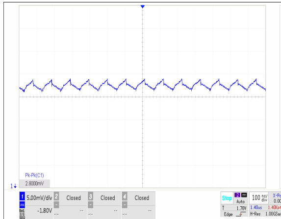
Figure 27. Output Voltage Ripple, V_{OUT} = 1.8V , Mode=High, I_{LOAD}=0A
