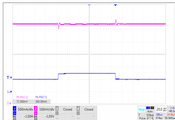
Figure 34. Load Transient, V_{OUT} = 1.8V , Mode=Low, I_{LOAD} = 500mA to 750mA
