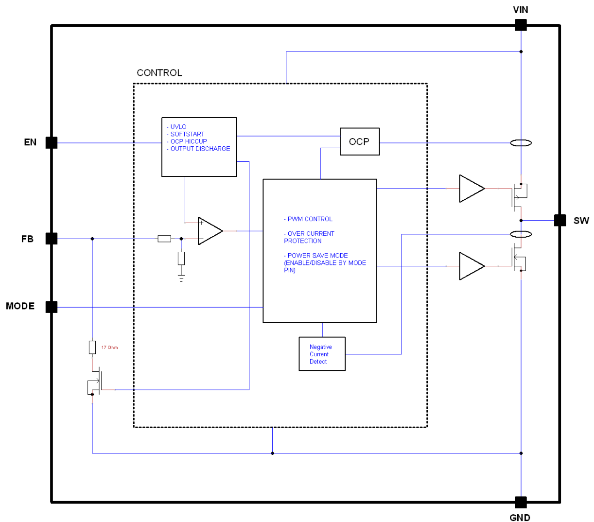
Figure 43. Block Diagram
