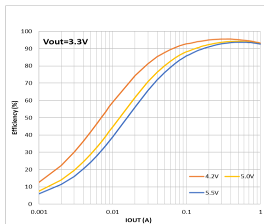
Figure 10. Efficiency, Mode=High, V_{OUT} = 3.3V
