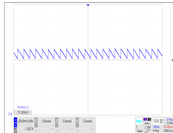
Figure 30. Output Voltage Ripple, V_{OUT} = 1.8V , Mode=Low, I_{LOAD}=0A
