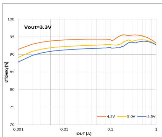
Figure 9. Efficiency, Mode=Low, V_{OUT} = 3.3V
