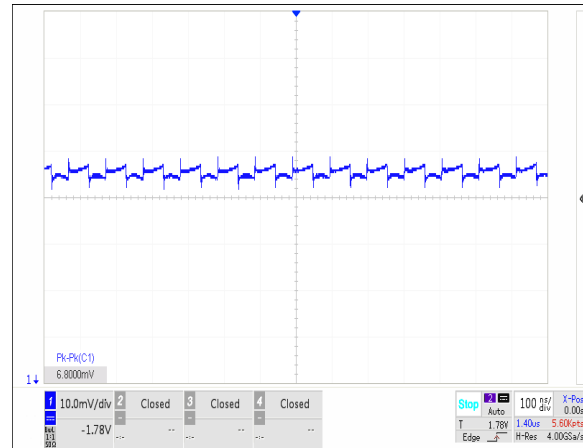
Figure 28. Output Voltage Ripple, V_{OUT} = 1.8V , Mode=High, I_{LOAD}=500mA
