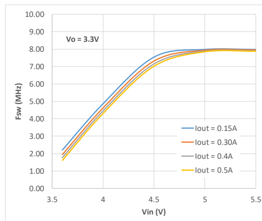
Figure 26. FSW, V_{OUT} = 3.3V , Mode=High
