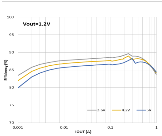
Figure 5. Efficiency, Mode=Low, V_{OUT} = 1.2V
