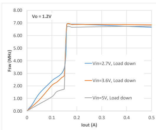
Figure 21. FSW, V_{OUT} = 1.2V , Mode=Low
