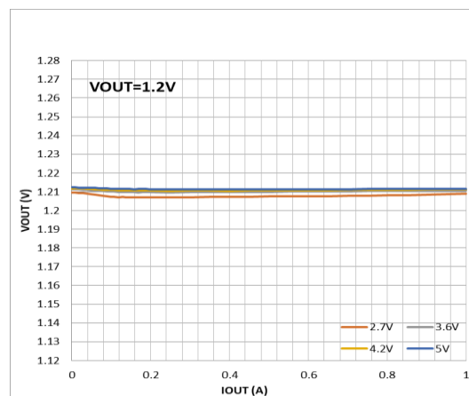
Figure 12. Load regulation, Mode=High, V_{OUT} = 1.2V
