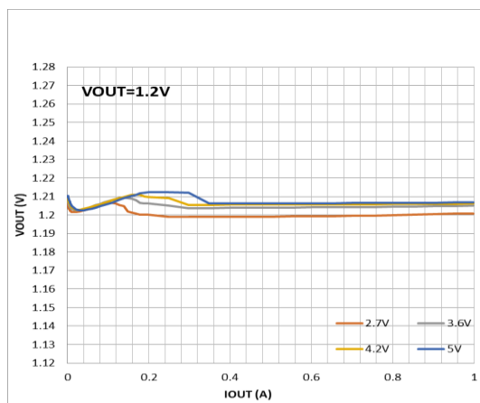
Figure 11. Load regulation, Mode=Low, V_{OUT} = 1.2V
