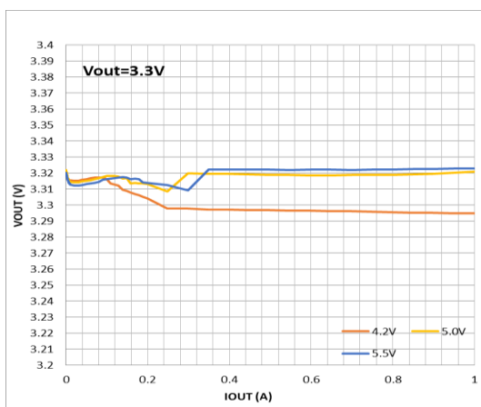
Figure 15. Load regulation, Mode=Low, V_{OUT} = 3.3V
