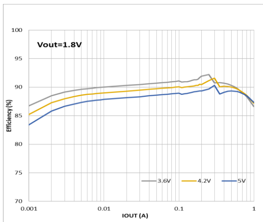
Figure 7. Efficiency, Mode=Low, V_{OUT} = 1.8V
