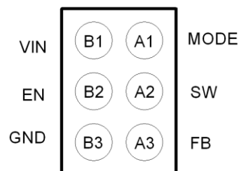
Figure 4. Bottom View
