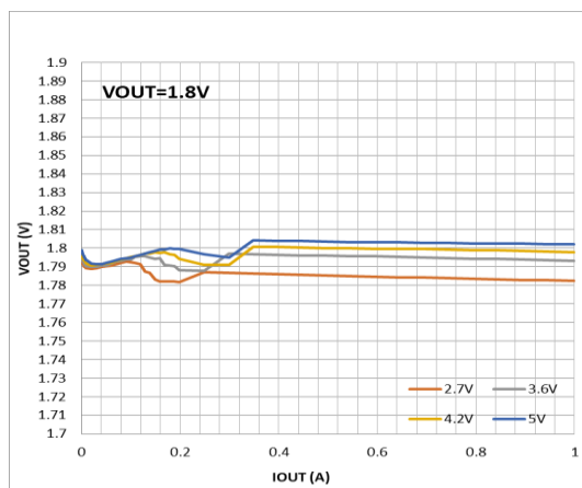
Figure 13. Load regulation, Mode=Low, V_{OUT} = 1.8V
