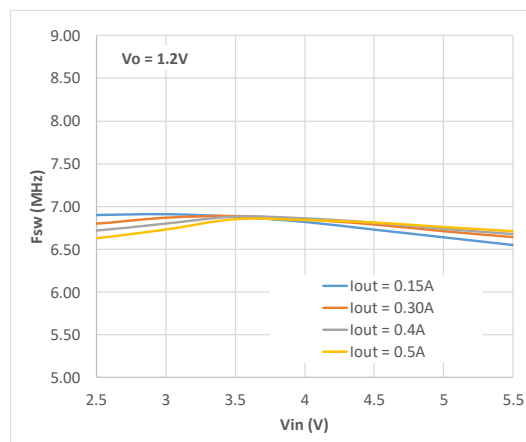
Figure 22. FSW, V_{OUT} = 1.2V , Mode=High
