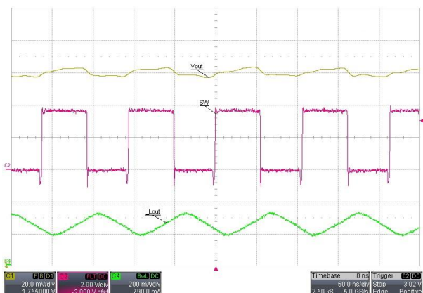
Figure 40. PWM Mode Operation: V_{IN} = 3.6V , V_{OUT} = 1.8V , I_{LOAD} = 300mA
