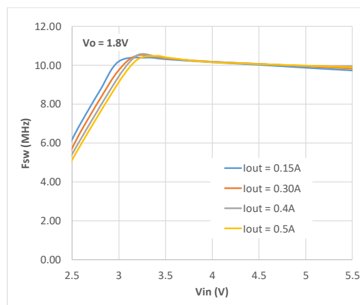
Figure 24. FSW, V_{OUT} = 1.8V , Mode=High
