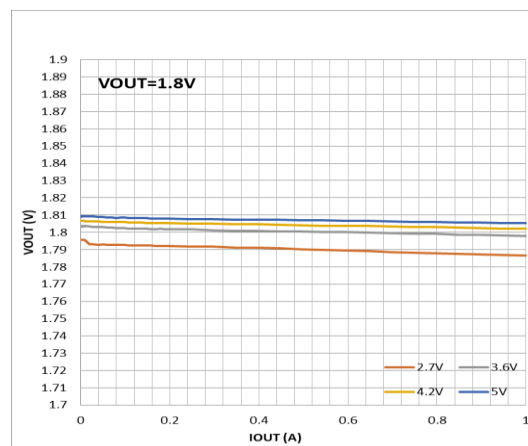
Figure 14. Load regulation, Mode=High, V_{OUT} = 1.8V
