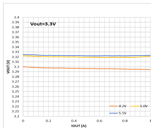
Figure 16. Load regulation, Mode=High, V_{OUT} = 3.3V
