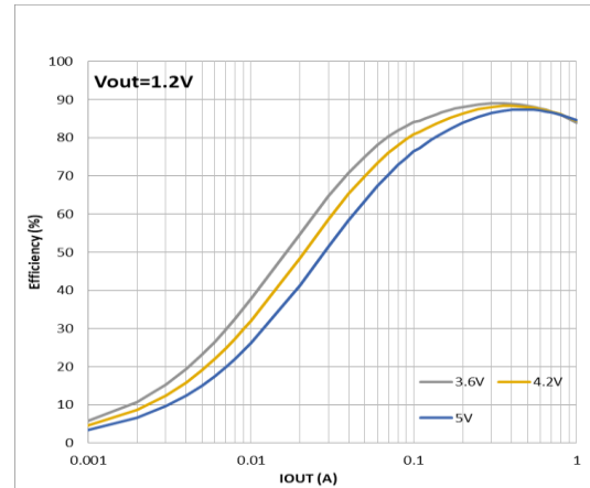
Figure 6. Efficiency, Mode=High, V_{OUT} = 1.2V
