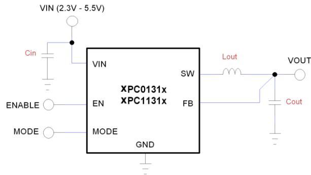
Figure 44. Application Circuit
