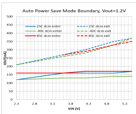
Figure 19. PFM/PWM Boundaries, Mode=Low, V_{OUT} = 1.2V
