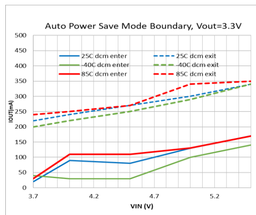
Figure 20. PFM/PWM Boundaries, Mode=Low, V_{OUT} = 3.3V
