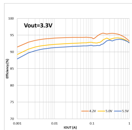
Figure 2. Typical Efficiency, Mode= Low
