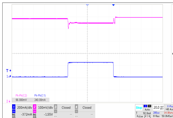
Figure 33. Load Transient, V_{OUT} = 1.8V , Mode=Low, I_{LOAD} = 0A to 250mA
