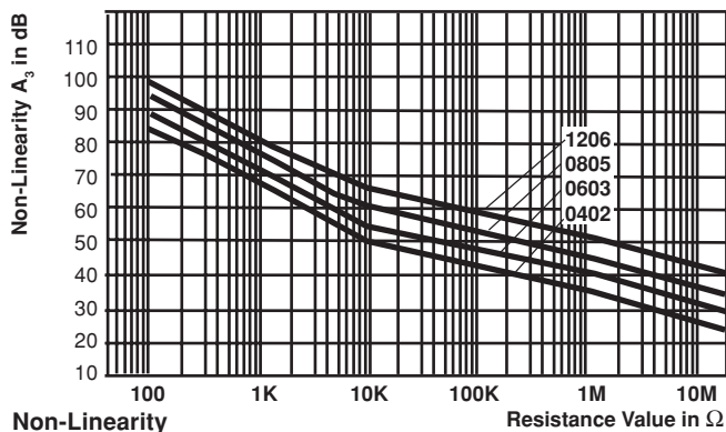
Non-Linearity
