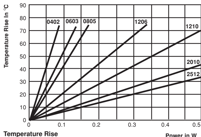
Temperature Rise
