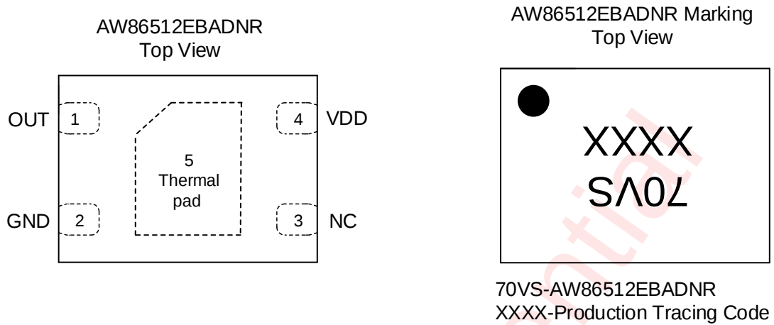
Figure 2 Pin Configuration And Top Mark
