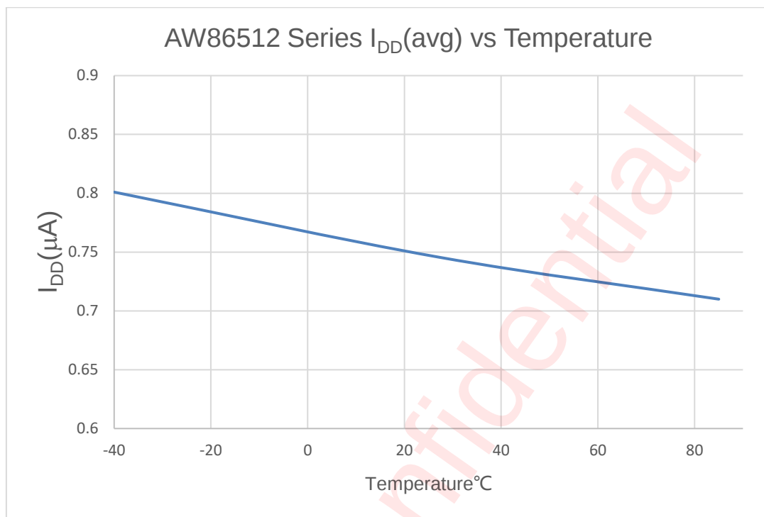
Ambient Temperature T_a[^{\circ}\text{C}] I_{DD} vs. T_a ( V_{DD}=1.8\text{V} )
