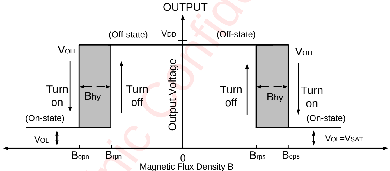
Figure 4 The Working Process of Omnipolar output
