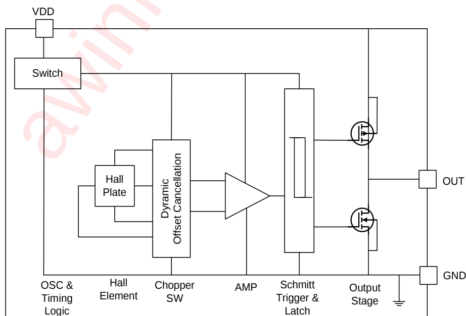
Figure 3 Functional Block Diagram of AW86512EBADNR
