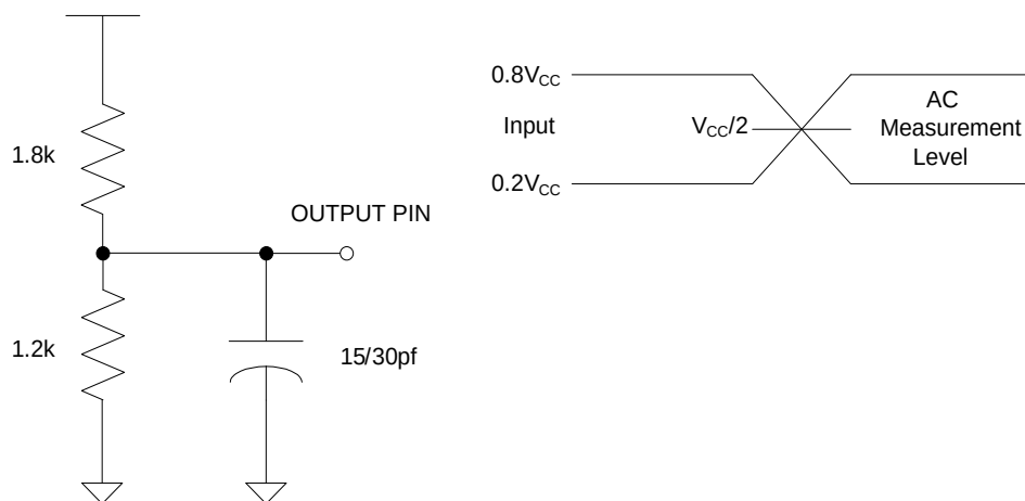
Figure 9.1 Output test load &amp; AC measurement I/O Waveform
