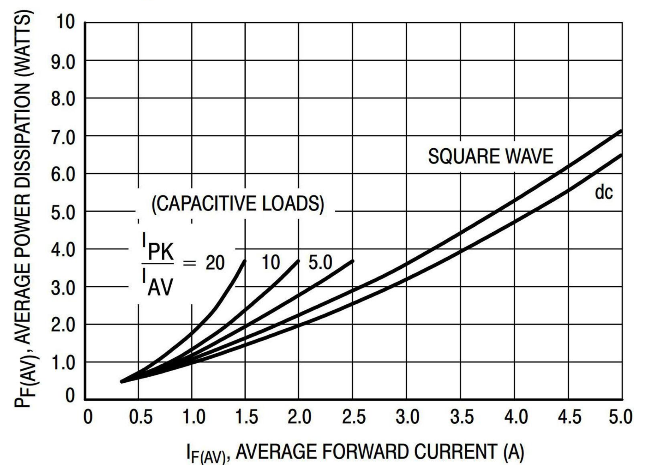
Figure 8. Power Dissipation
