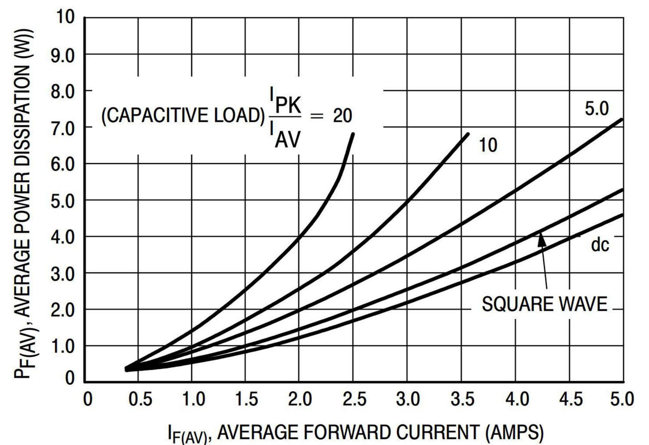
Figure 3. Power Dissipation
