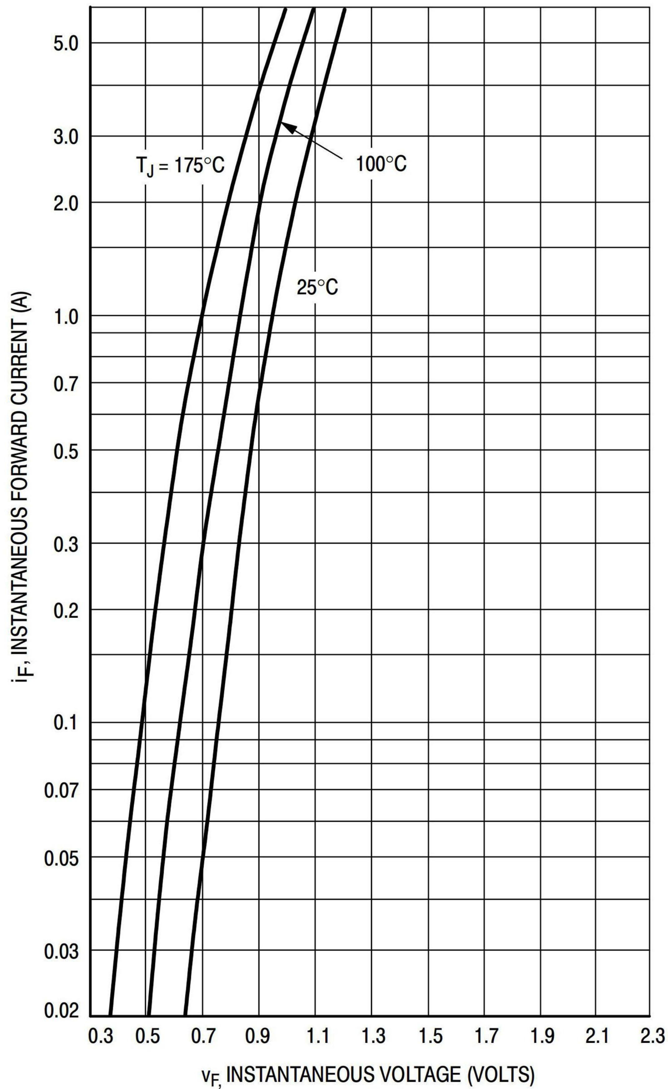
Figure 6. Typical Forward Voltage
