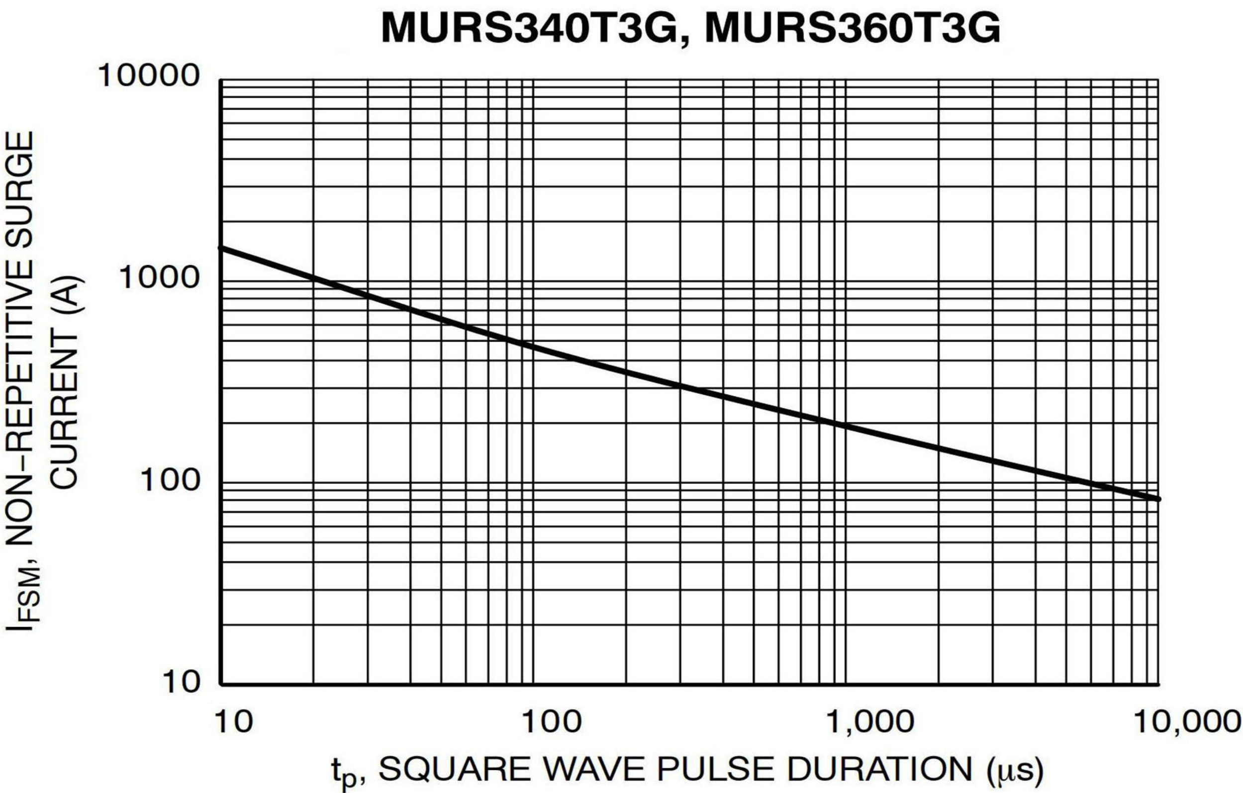
Figure 11. Typical Non-Repetitive Surge Current
