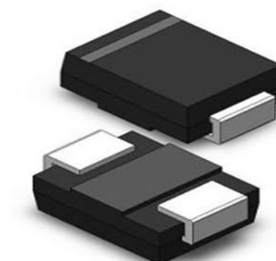
SMC 2-LEAD CASE 403AC
