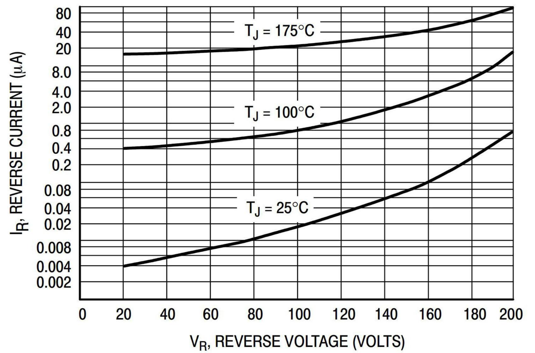
Figure 2. Typical Reverse Current*
