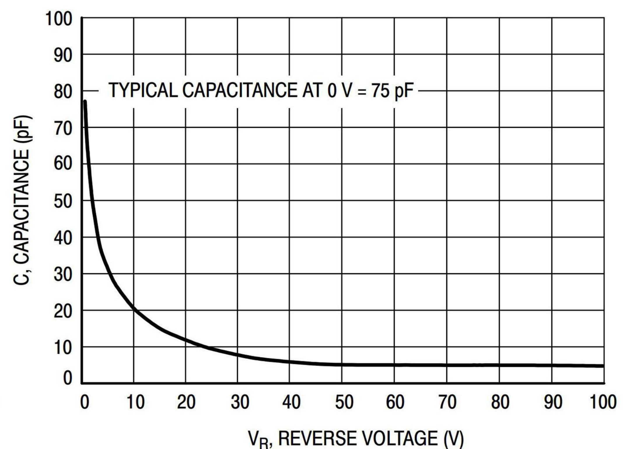
Figure 10. Typical Capacitance
