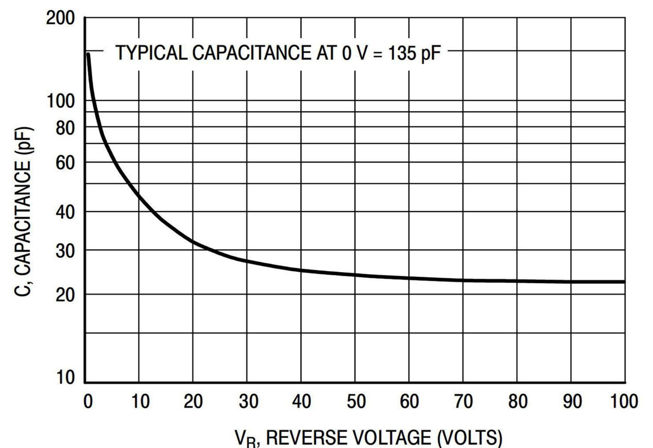
Figure 5. Typical Capacitance
