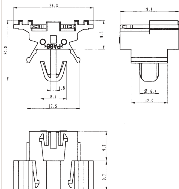
Fixing clip - AB02SFT
