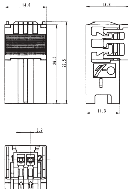
Male housing
