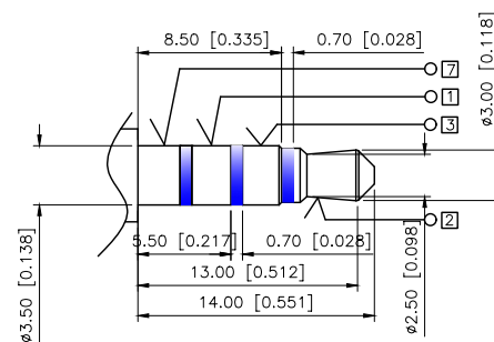
Matching Plug
